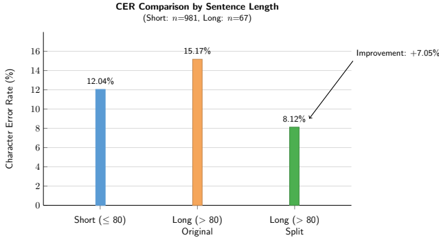
Fig. 4: CER comparison showing the effect of conjunction based splitting. Long sentences ( >80 chars) degrade to 15.17% CER when processed whole, but splitting at conjunction boundaries reduces error to 8.12%, even better than short sentences (12.04%).
