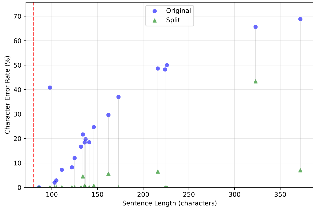
Split vs Original for Long Sentences
