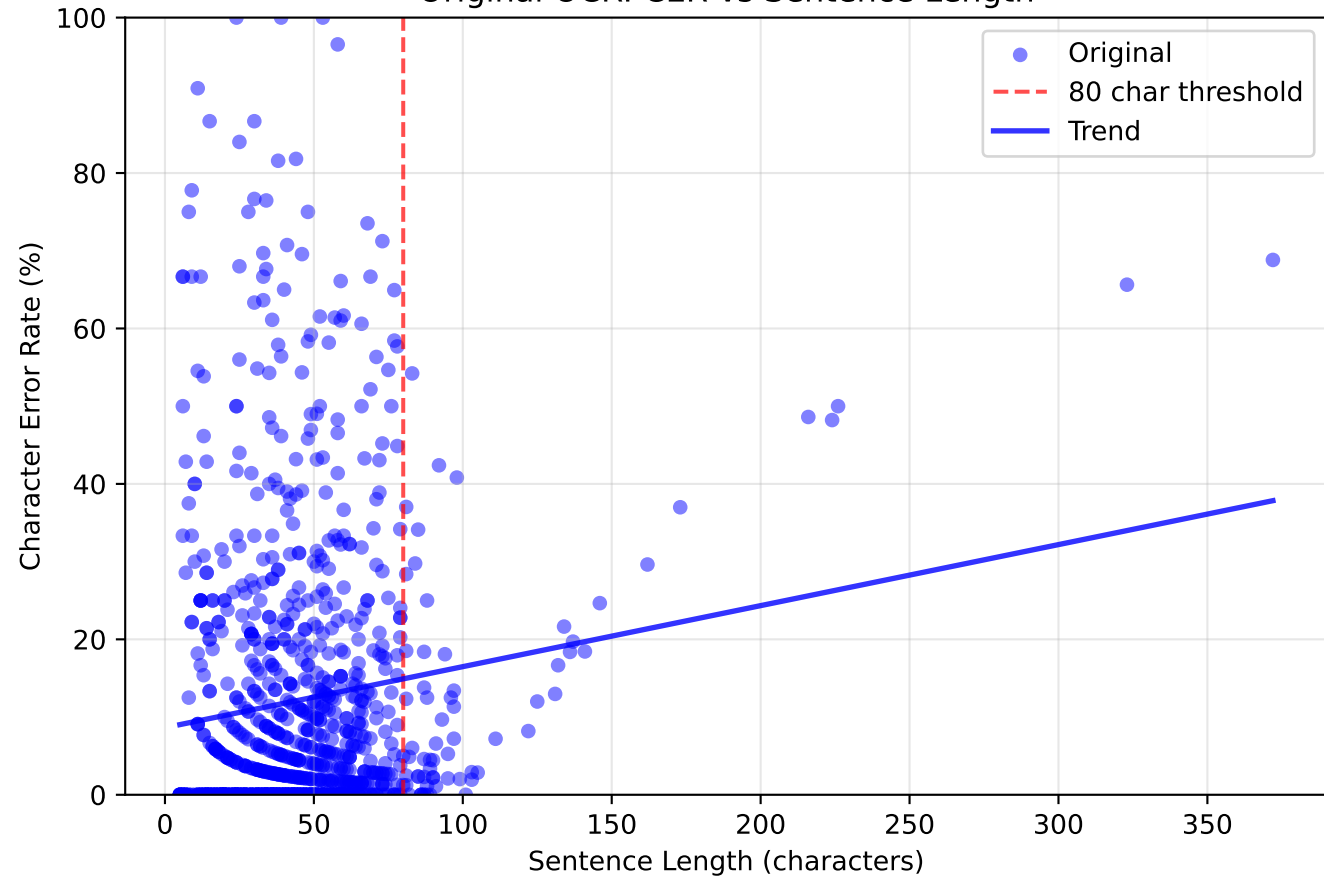
Original OCR: CER vs Sentence Length
