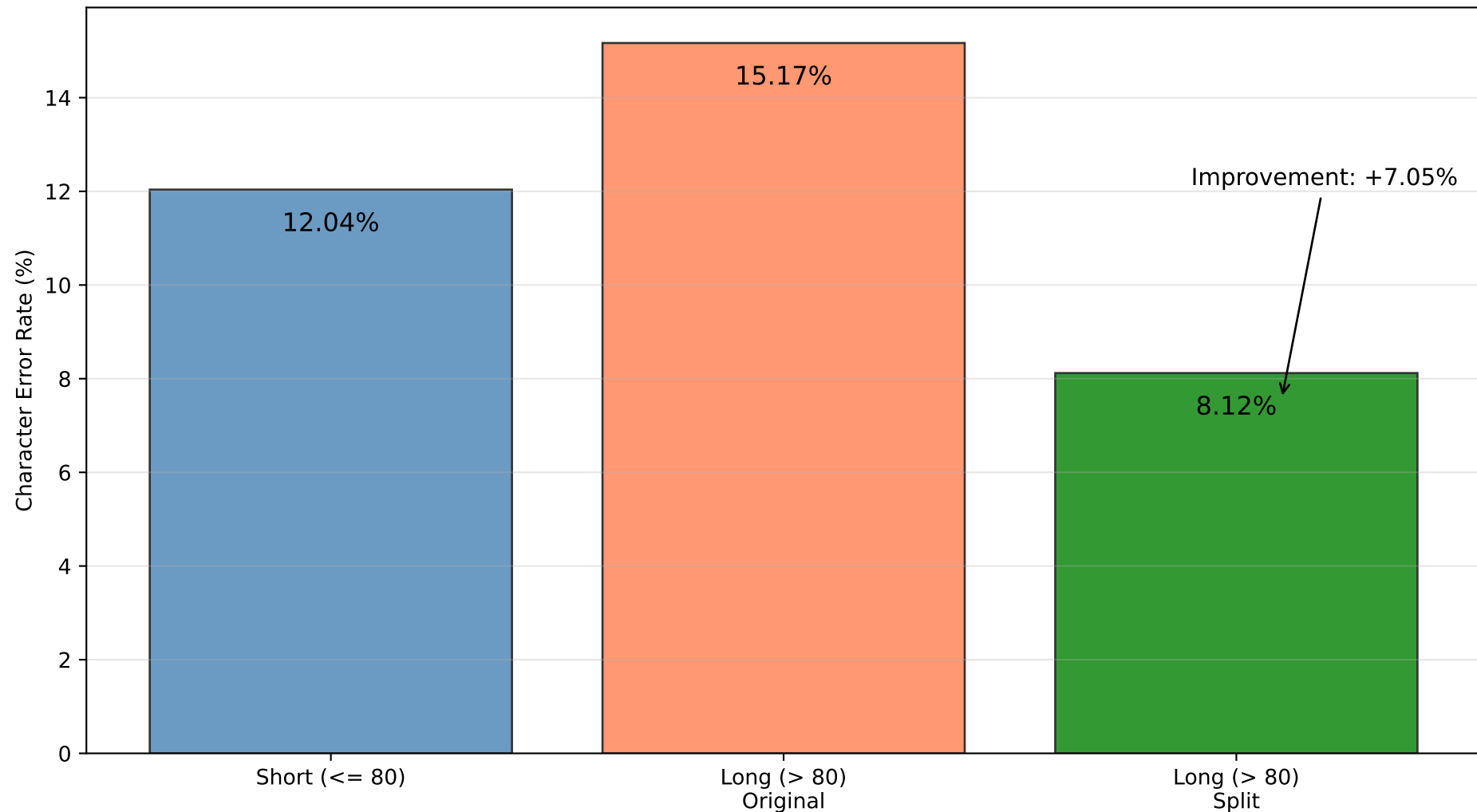
CER Comparison by Sentence Length (Short: n=981, Long: n=67)
