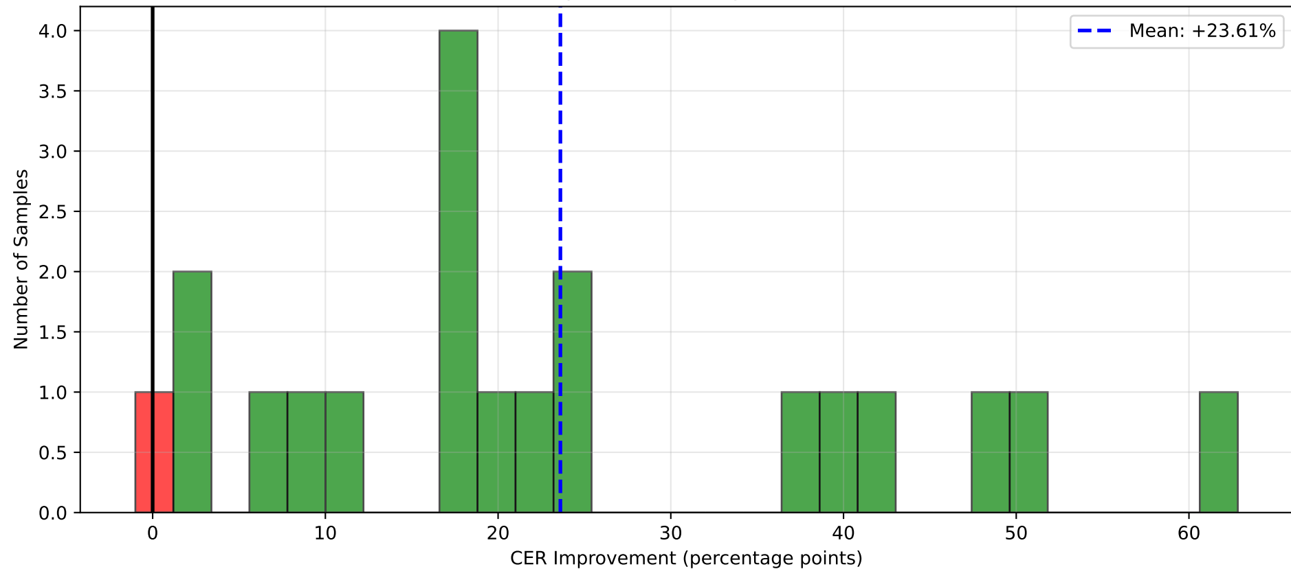
CER Improvement Distribution for Split Sentences (Improved: 19, Degraded: 0)
