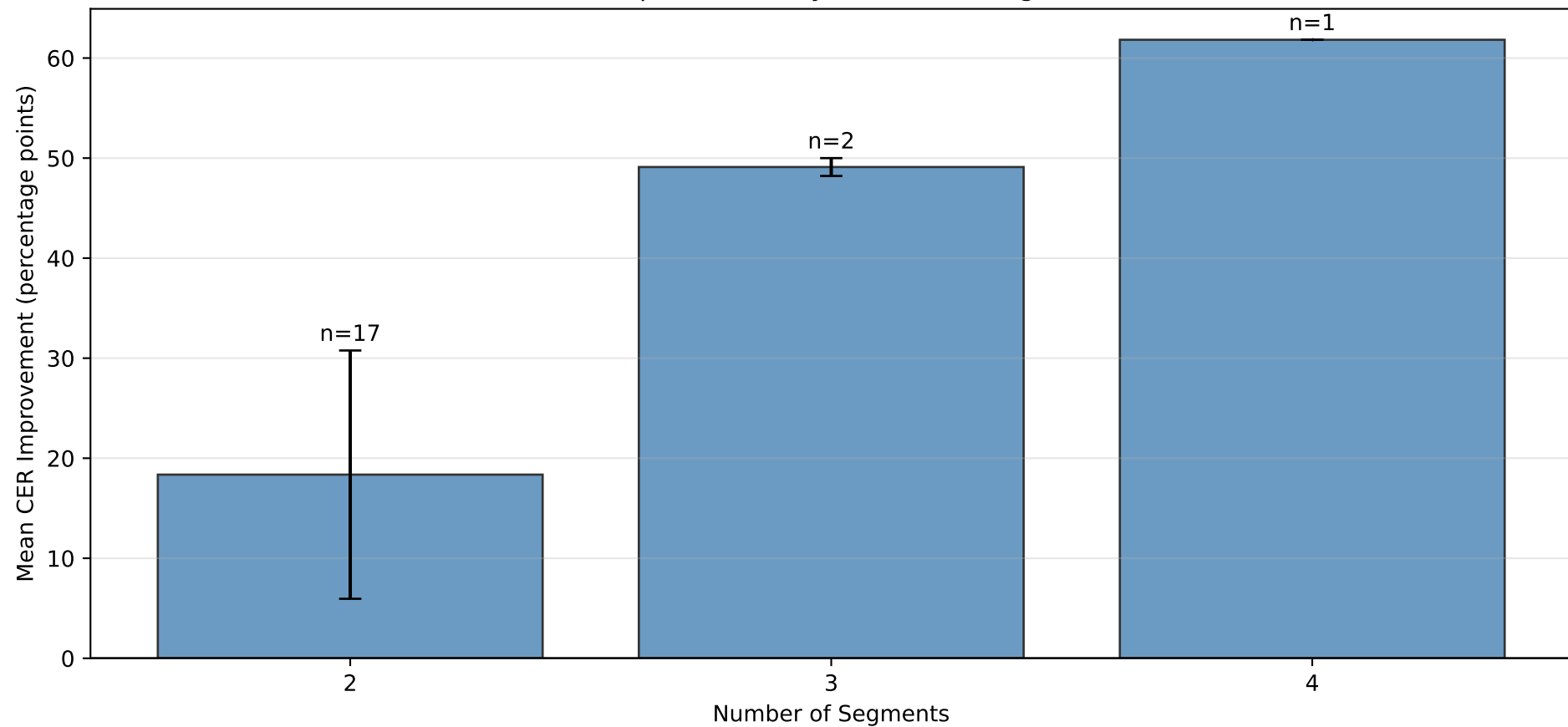
CER Improvement by Number of Segments
