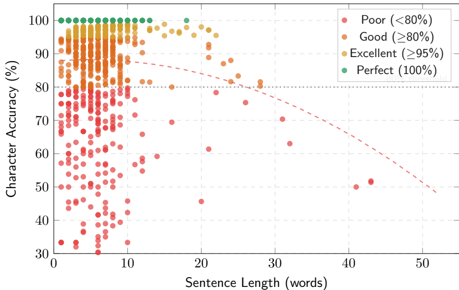
OCR Character Accuracy vs. Sentence Length
