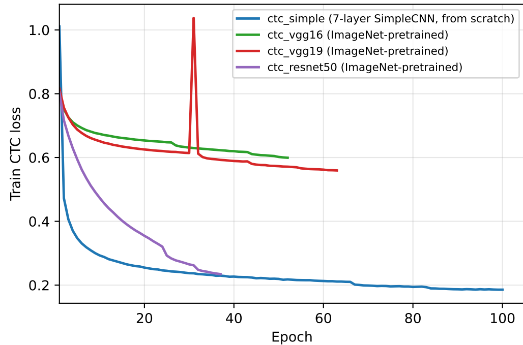
Training loss vs. epoch
