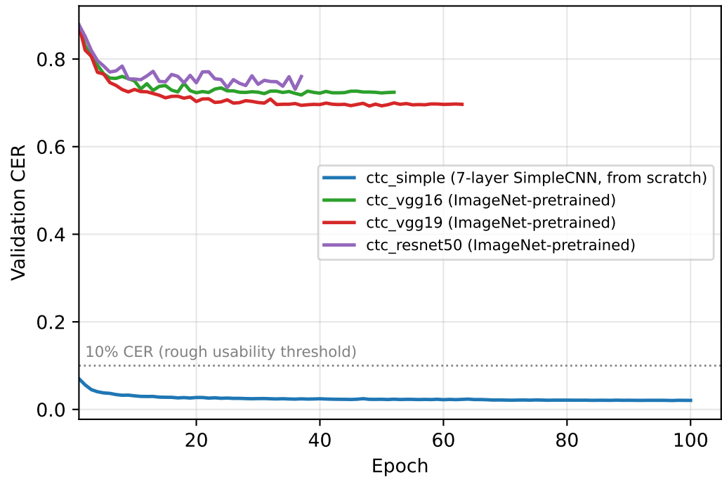
Validation CER vs. epoch
