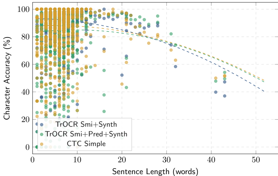
Model Comparison: Accuracy vs. Sentence Length
