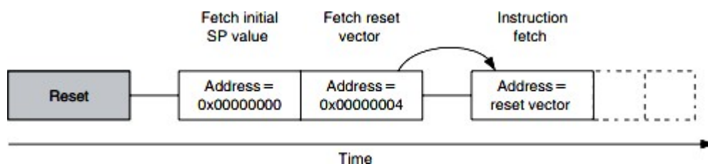
Figure 3.Reset sequence
