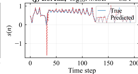
(j) Lorenz, \log_{10}\text{NMSE} = -0.51
