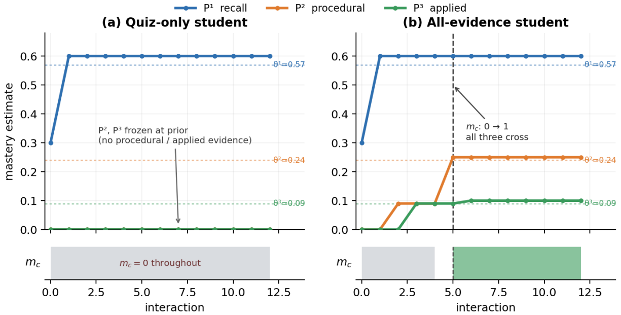
Fig. 6: Mastery trajectories from the update equations. A quiz-only student (a) drives the recall estimate to its ceiling while the procedural and applied estimates remain at their priors, so m_c = 0 throughout. A student supplying all three evidence types (b) is certified ( m_c: 0 \rightarrow 1 ) only once every dimension clears its threshold.
