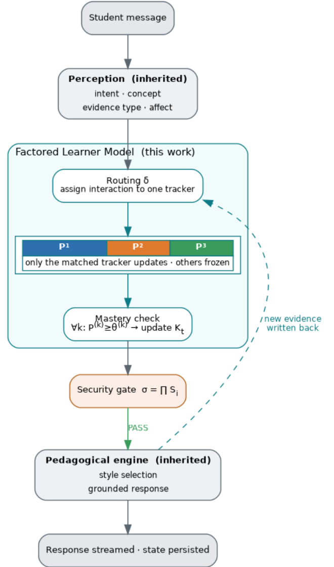
Fig. 3: Processing pipeline for a single interaction. The contribution (tinted) routes each interaction to one tracker, re-evaluates mastery, and updates K_t ; only requests passing the security gate reach the pedagogical engine, which writes new evidence back to the learner model.
