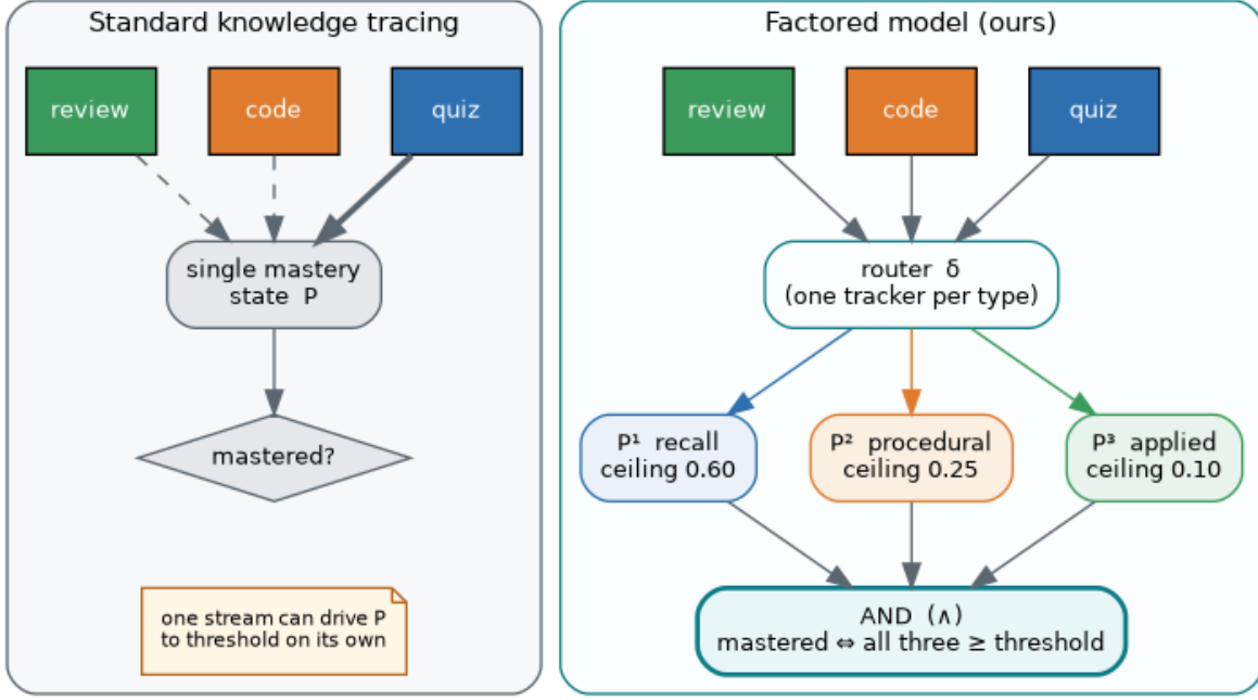
Fig. 4: Single-stream versus factored mastery. Standard knowledge tracing pools all evidence into one estimate (left), so a single stream can drive it to threshold; the factored model routes each evidence type to its own capped tracker and certifies mastery only when all three clear threshold (right).
