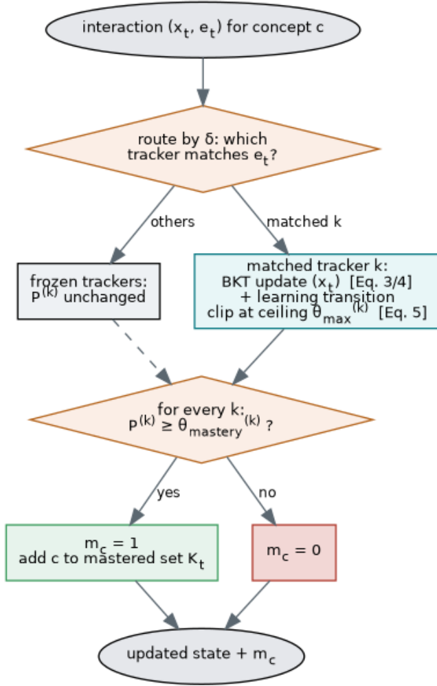
Fig. 5: Per-interaction update. Routing \delta selects the one tracker matching the evidence type; the matched tracker applies the BKT update and ceiling clip while the others are frozen; mastery is the conjunction of three threshold tests, and a satisfied concept enters the mastered set K_t .
