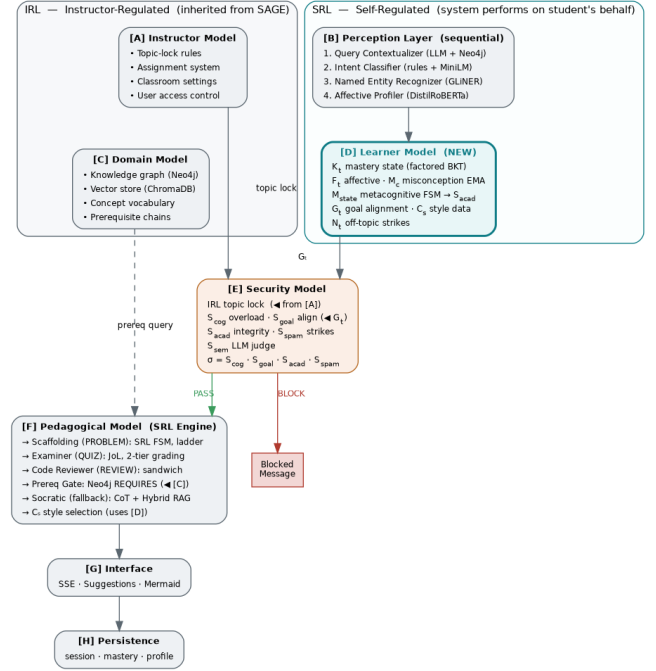
Fig. 2: System architecture. The instructor-regulated track (grey, inherited from SAGE) sets curriculum boundaries; the self-regulated track maintains per-student state. The factored learner model (D, highlighted) is the contribution; the gate, pedagogical engine, and infrastructure are inherited. All processing flows through the gate that consumes the mastered set K_t .
