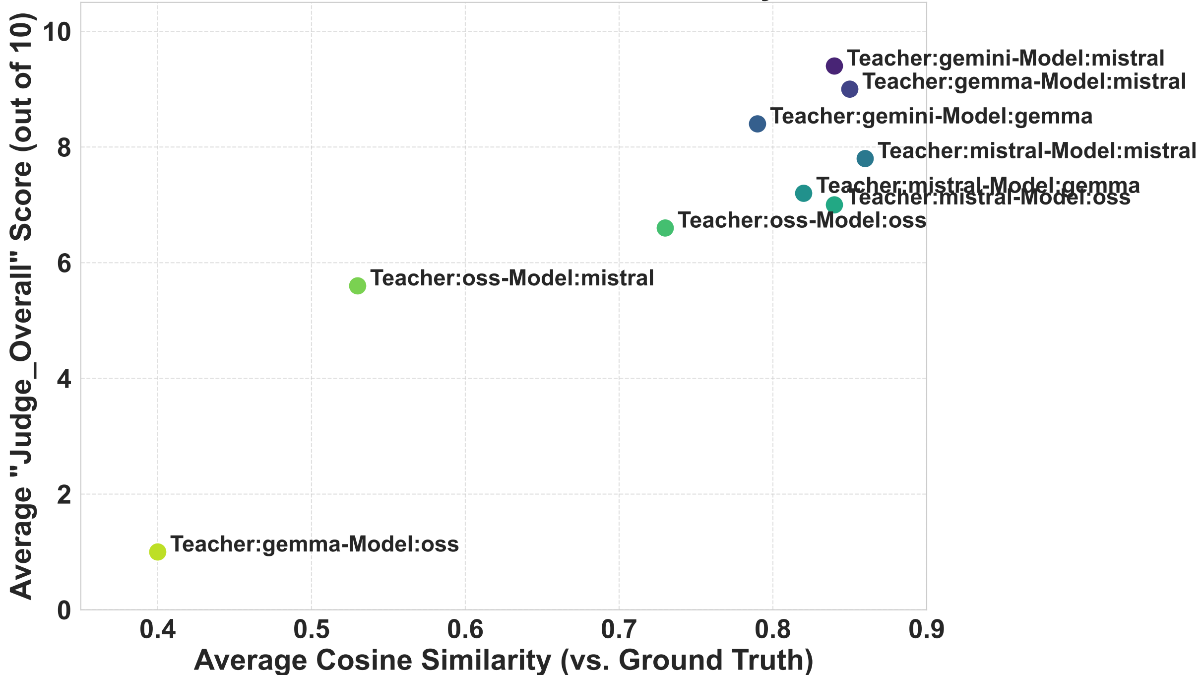
Performance vs. Semantic Similarity
