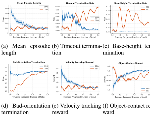
Figure 4: TD3 vs PPO in the obstacle world no LiDAR ablation. The additional object contact reward captures the obstacle collision penalty. This setting evaluates robustness to contact-rich interactions under partial observability.
