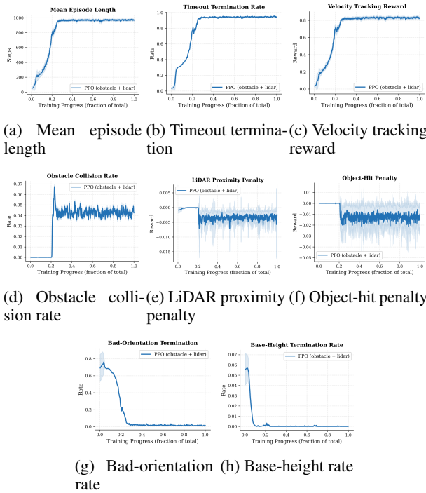
Figure 6: Ablation IV: PPO+LiDAR training in the dense obstacle world (fine-tuned from the empty-world checkpoint). The policy reaches a 94.5% timeout rate and a 4.2% collision rate, with the LiDAR proximity penalty driving anticipatory obstacle avoidance before physical contact. TD3+LiDAR results are omitted as the robot falls immediately throughout training (see Figure 5).
