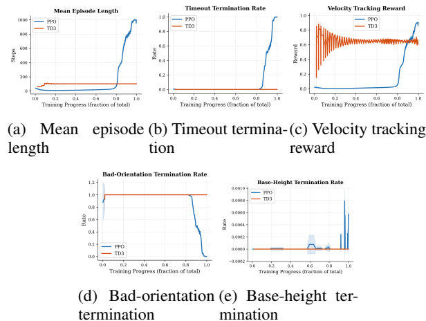
Figure 5: Ablation III: TD3 vs. PPO in the empty world with LiDAR observations. PPO converges to near-maximal episode length while TD3 immediately falls throughout all 5 M training steps, demonstrating that serial off-policy collection cannot learn from 1,720-dimensional LiDAR inputs.
