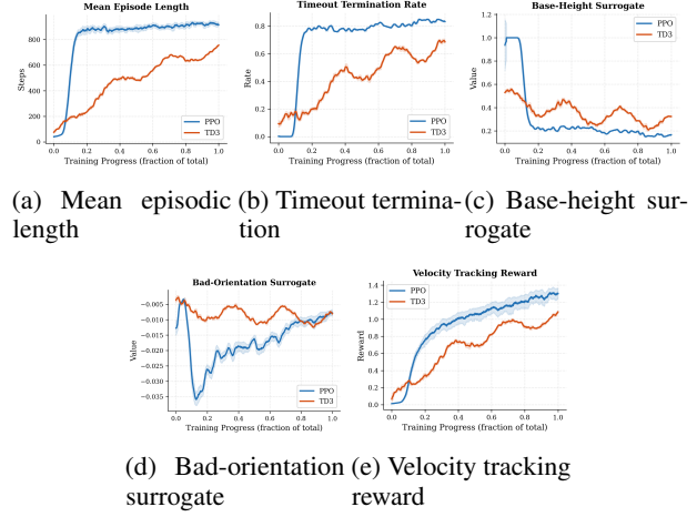
Figure 3: TD3 vs PPO in the empty-world no-LiDAR ablation. Curves show dense training traces with rolling mean and one-standard-deviation bands. This setting isolates locomotion stability and command following without obstacle contacts.
