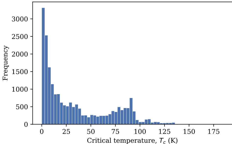
Distribution of superconducting critical temperature
