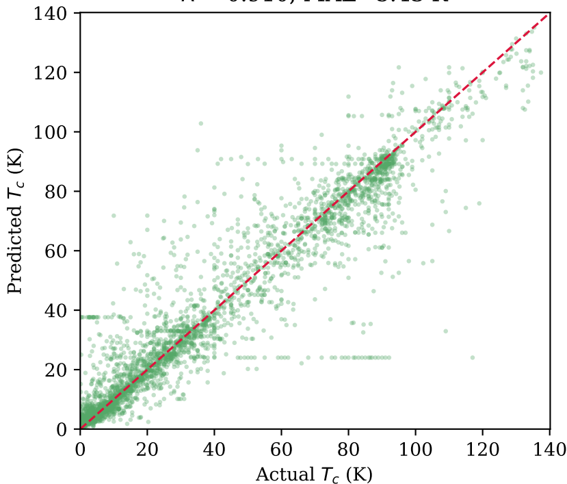
Parity plot, held-out set (Extra Trees) R^2=0.910 , MAE=5.43 K
