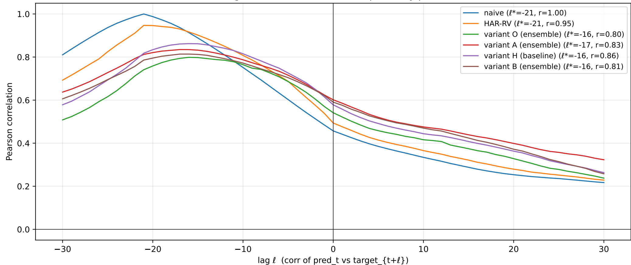
F1 diagnostic — cross-correlation profile by predictor
