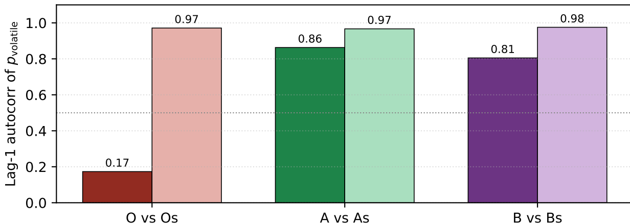
(b) Regime persistence on the test window (higher = more persistent regimes)
