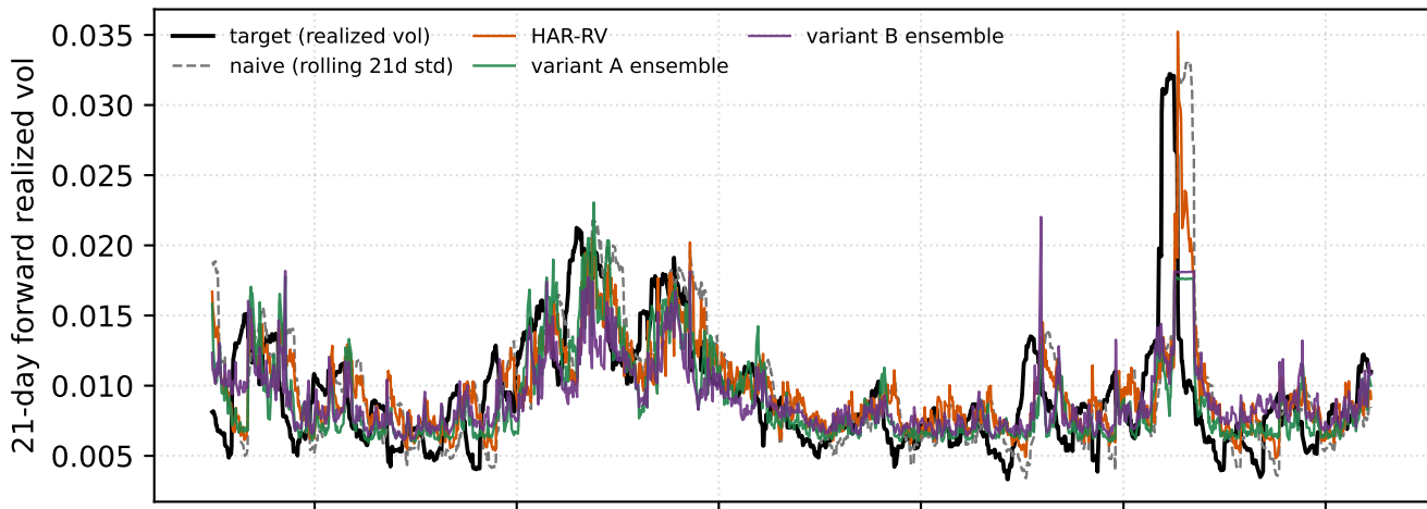
(a) Forecasts vs realized vol on the 1,440-day common test window
