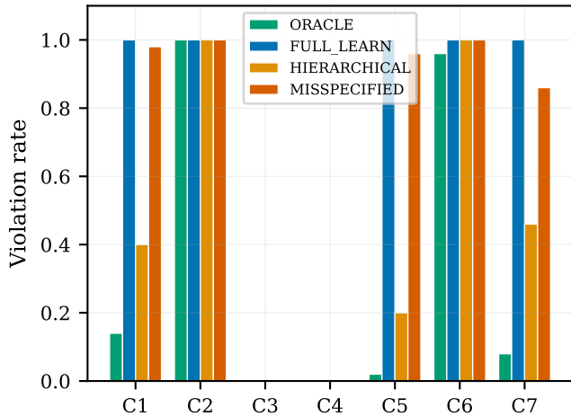
(b) Violation rate by A-matrix source
