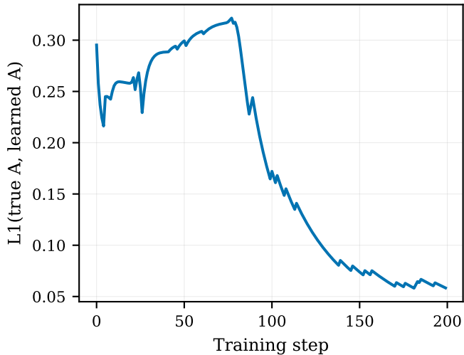
(a) A-matrix learning curve
