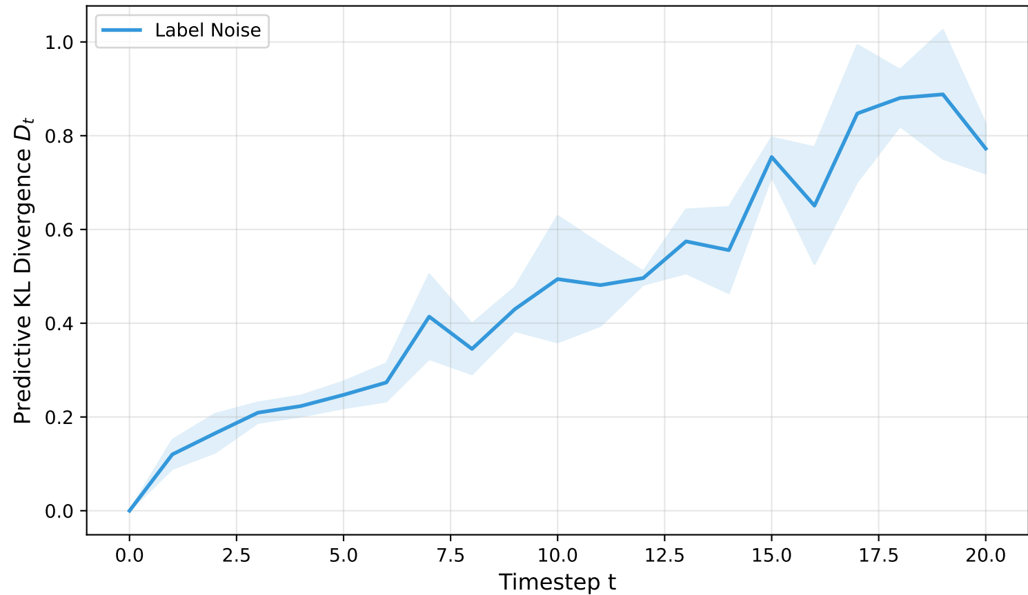
Drift Accumulation Over Time
