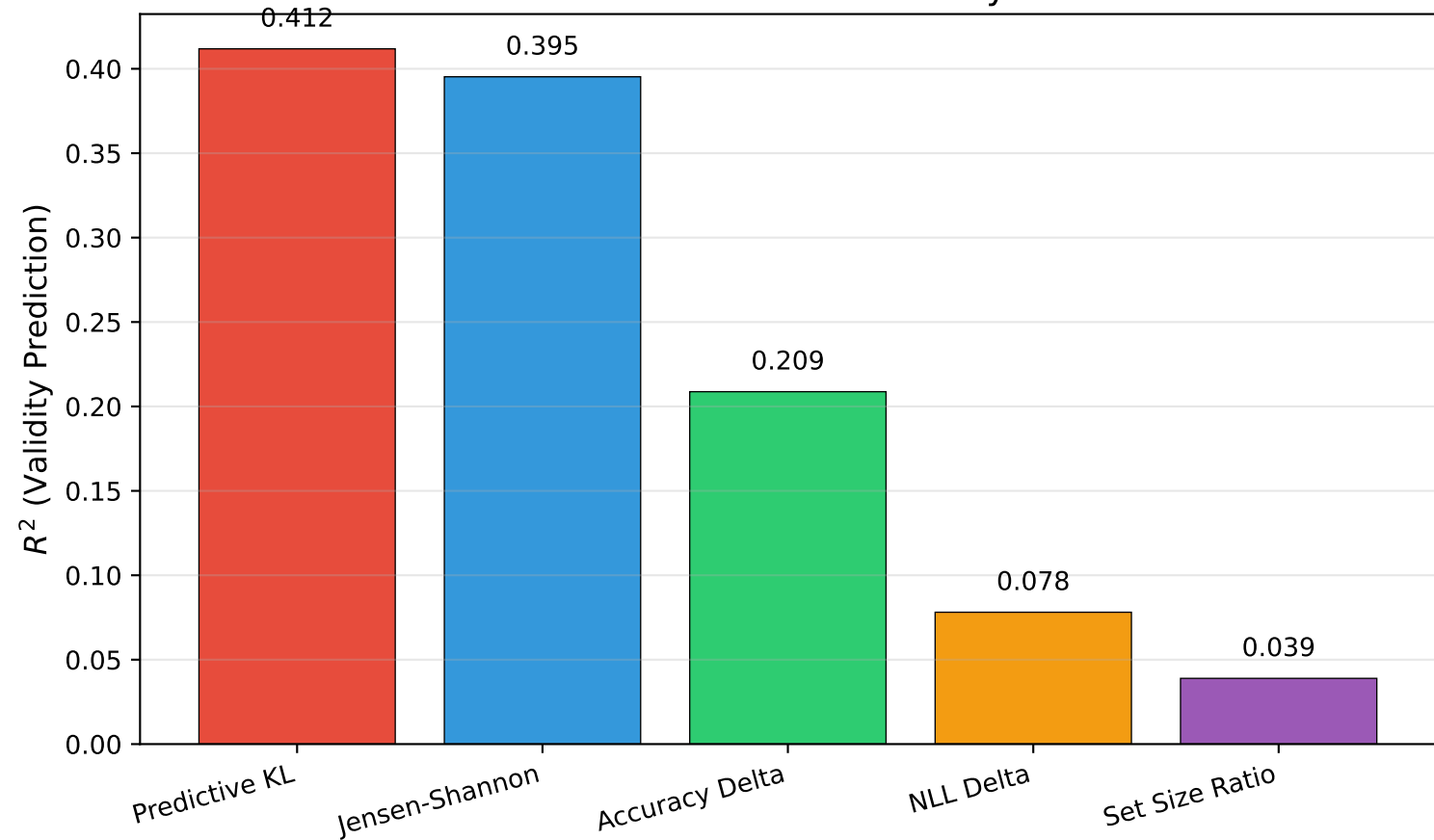
Ablation: Drift Measures as Validity Predictors
