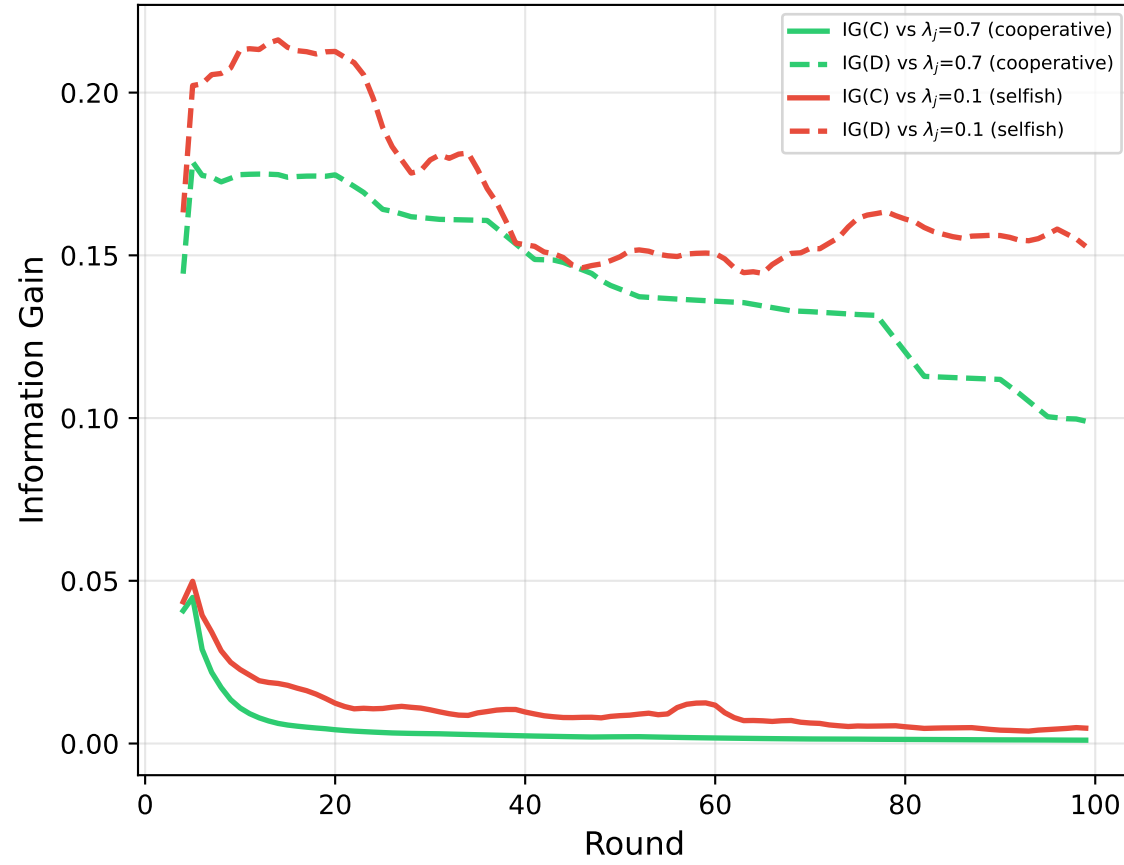
B. Epistemic value over time
