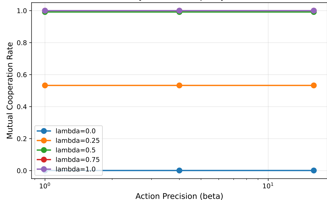
Effect of Beta on Cooperation (Symmetric Empathy)
