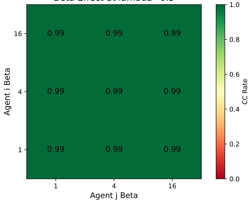
Beta Effect at \lambda=0.5
