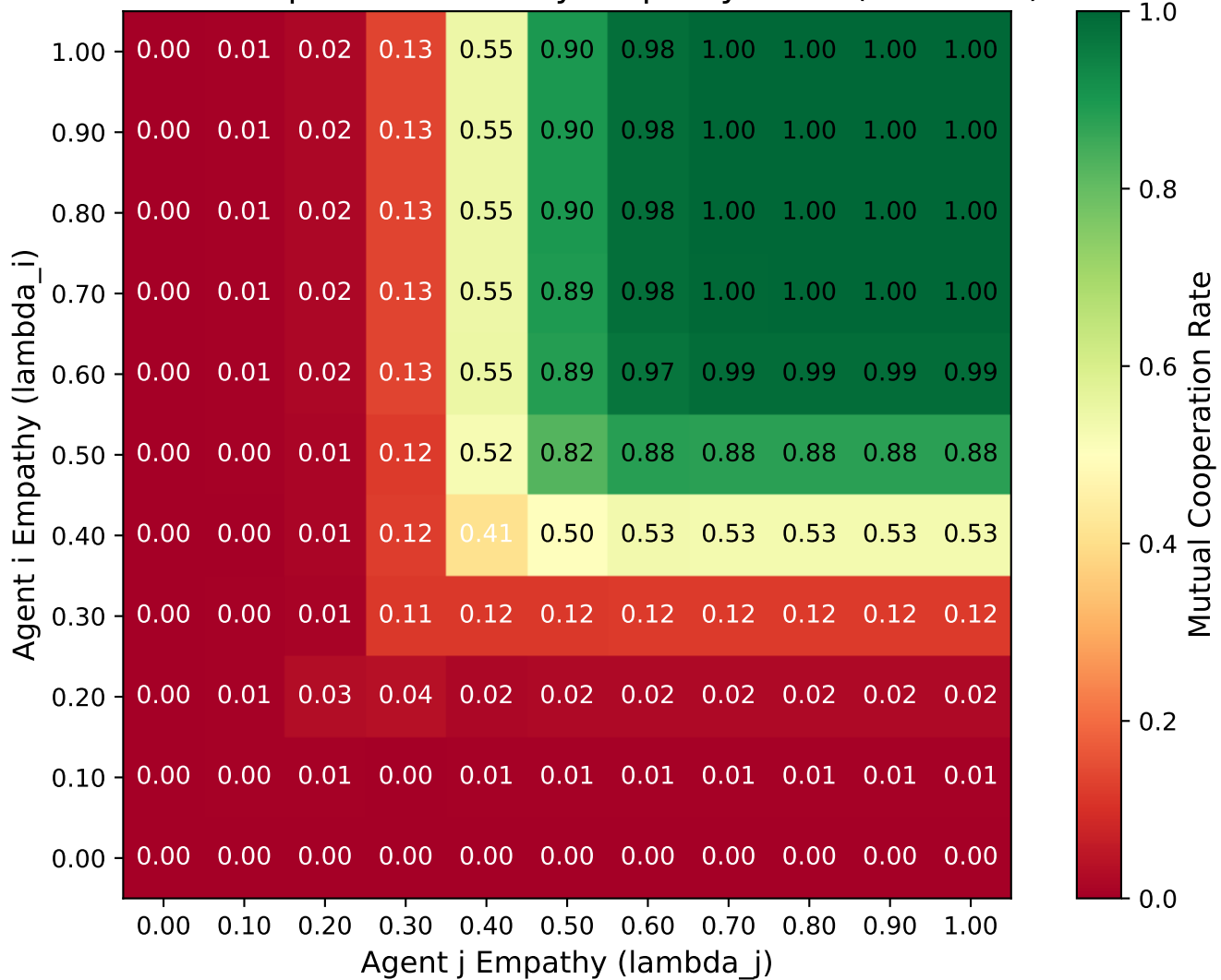
Mutual Cooperation Rate by Empathy Level (beta=4.0)
