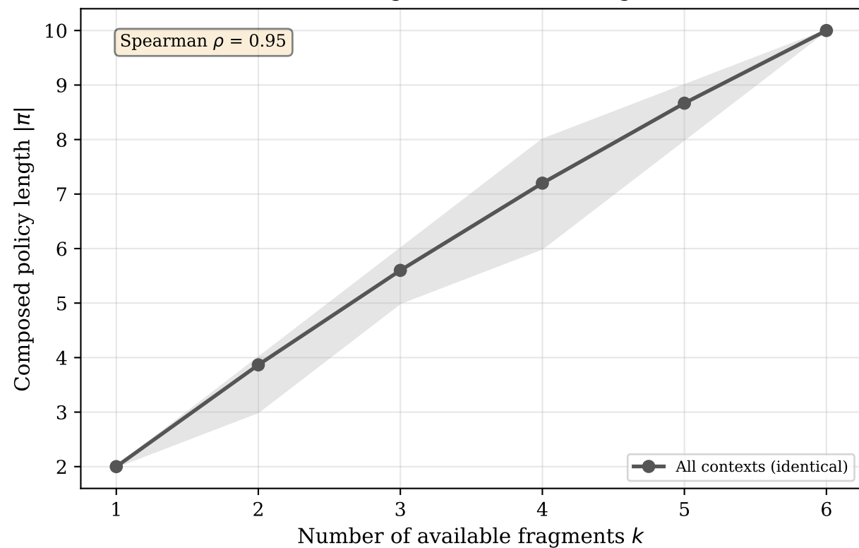
Policy Structure (Context-Invariant) Same fragments \rightarrow same length
