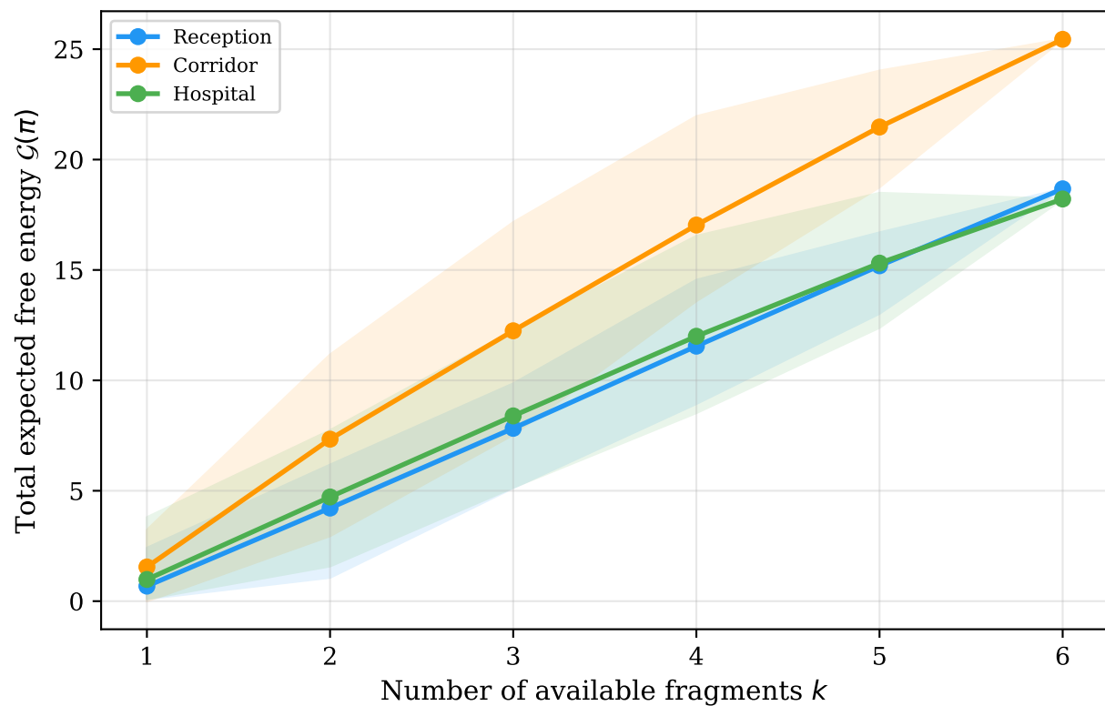
Policy Evaluation (Context-Dependent) Same structure \rightarrow different EFE
