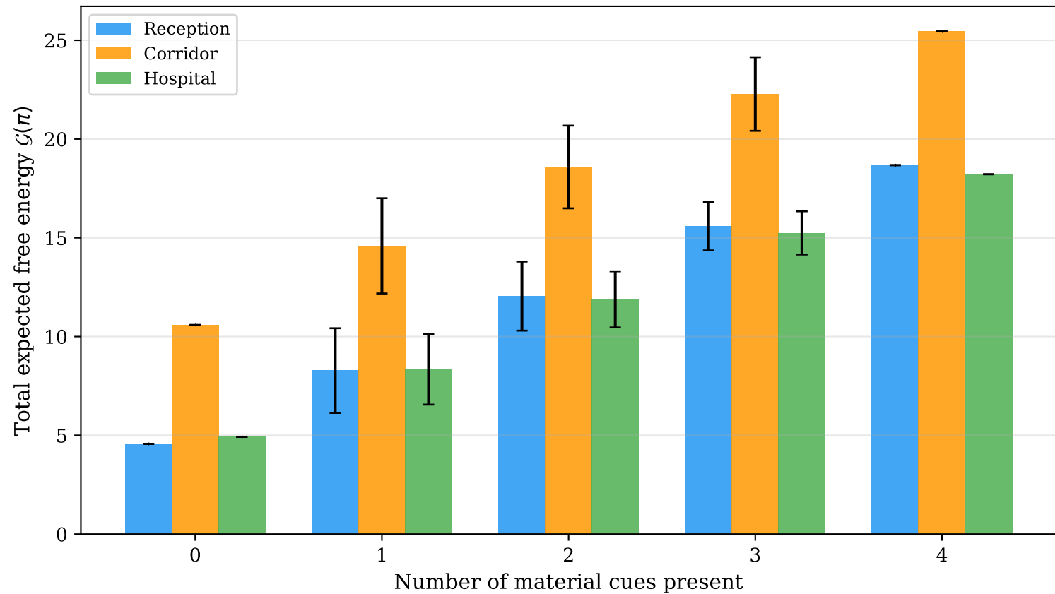
C-matrix Reshapes Policy Evaluation (Same policy structure, different free energy profiles)
