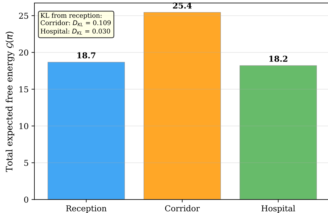
EFE Under Identical Knowledge Base (Same A/B, different C-matrix)
