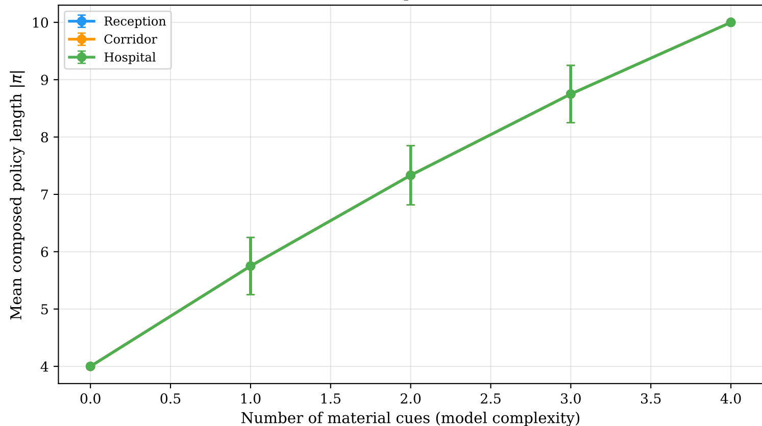
Context \times Model Complexity Interaction (C-matrix modulates response to model structure)
