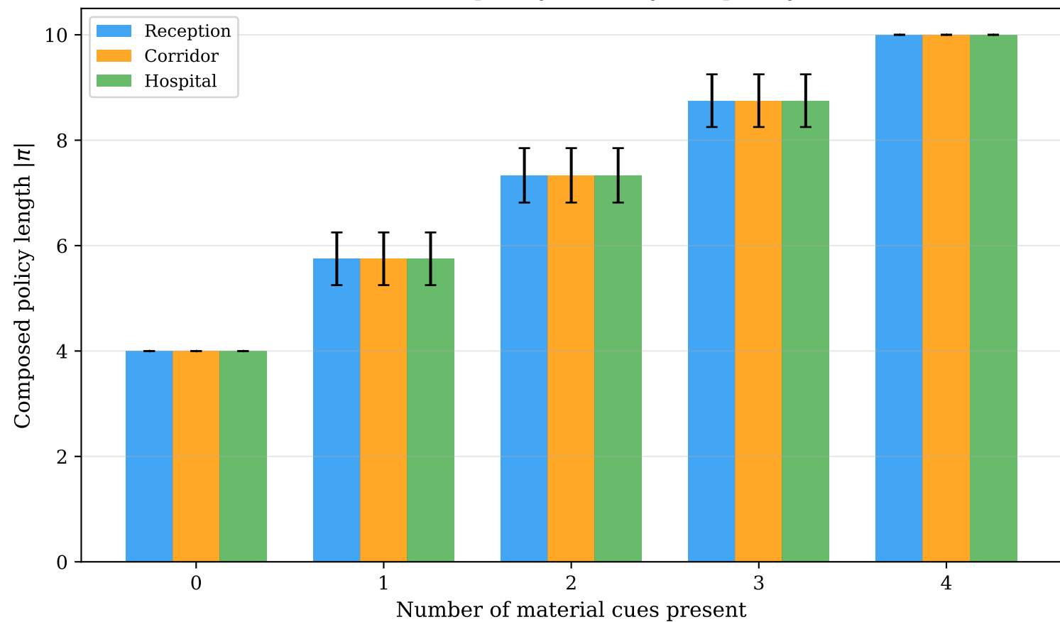
Model Complexity \rightarrow Policy Complexity
