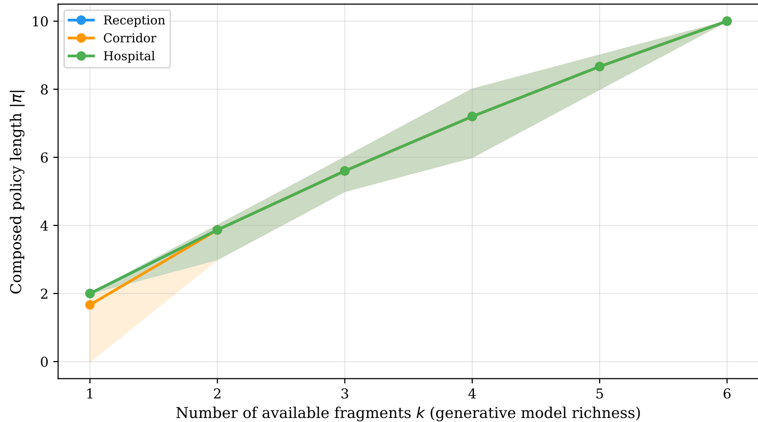
Graceful Degradation Under Model Sparsity (Variational inference minimizes F with available structure)
