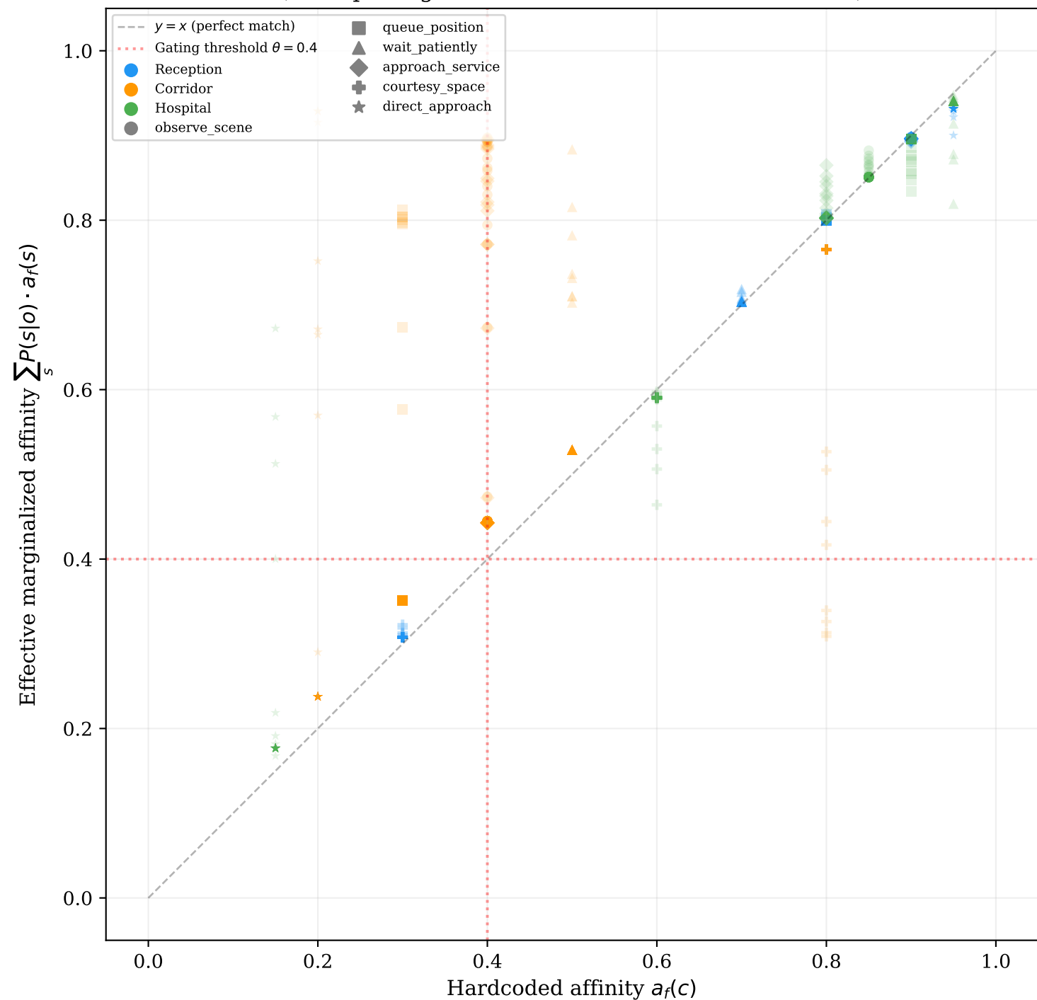
Effective vs. Hardcoded Fragment Affinity (Perception-grounded inference vs. oracle context)
