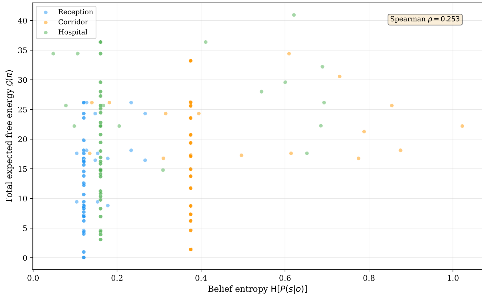
Perceptual Uncertainty vs. Policy Free Energy (Does A-matrix uncertainty propagate to policy evaluation?)
