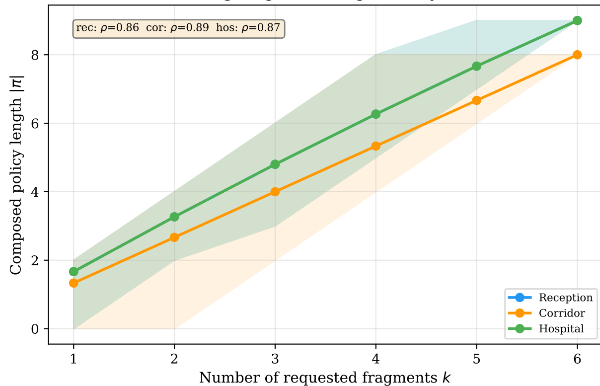
Policy Structure (Context-Dependent) D-matrix gating filters fragments by context
