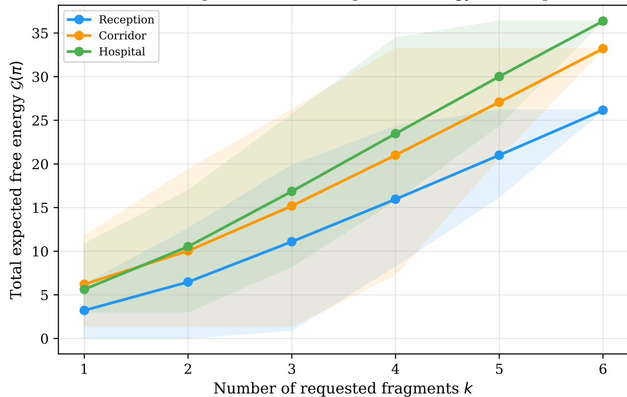
Policy Evaluation (Context-Dependent) C-matrix preferences reshape free energy landscape
