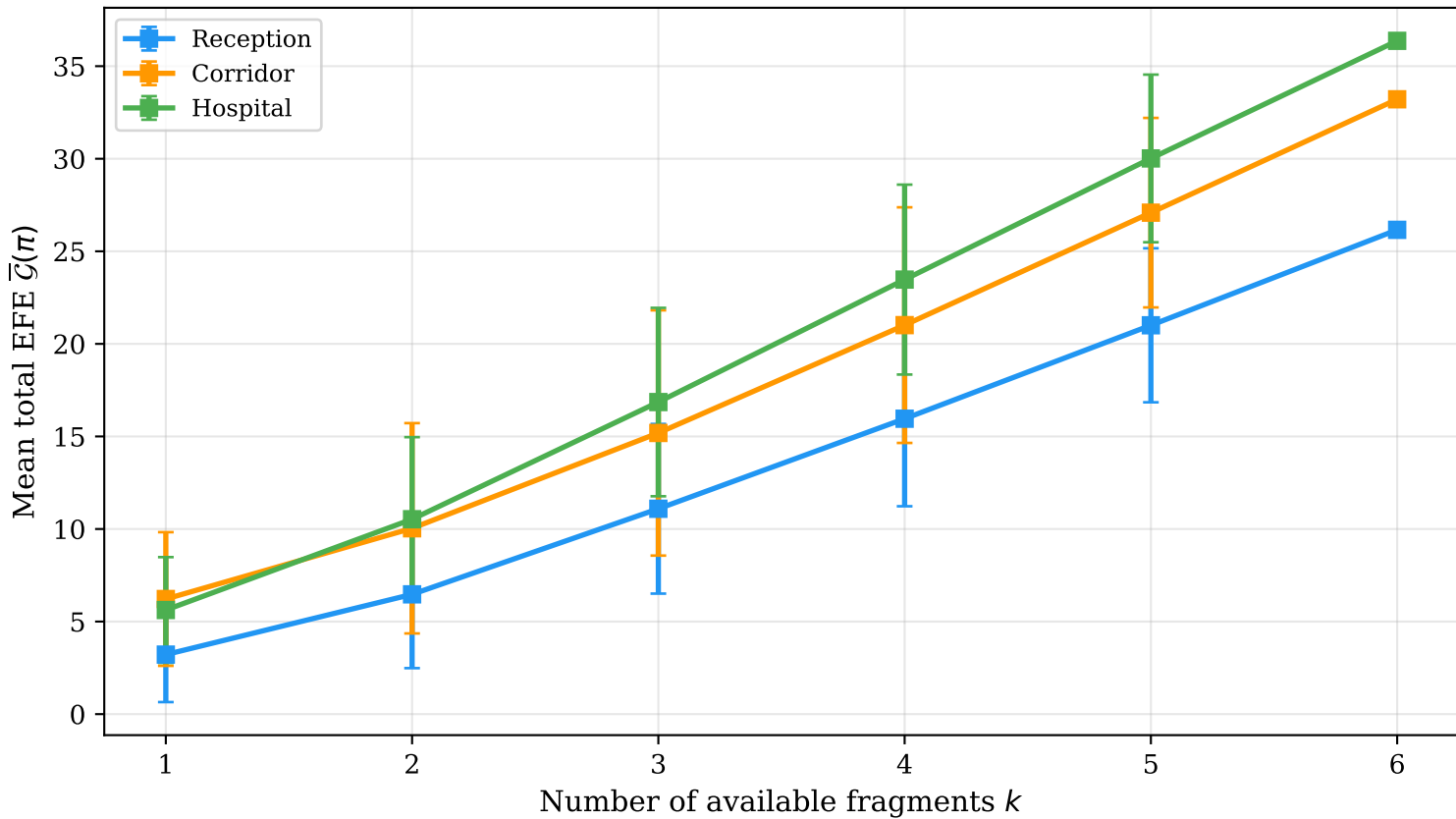
Expected Free Energy vs. Model Richness (Context preference structure creates persistent EFE separation)
