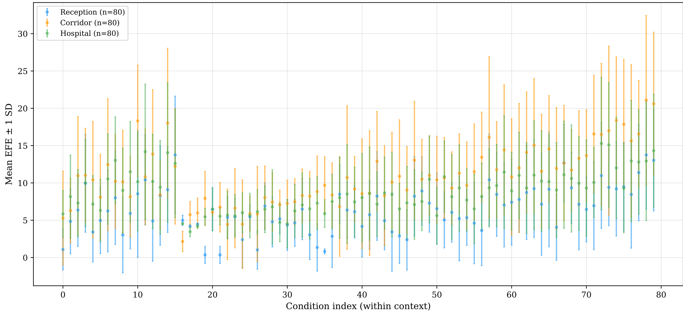
Per-Condition EFE Distributions (Error bars show real variance from stochastic gating)
