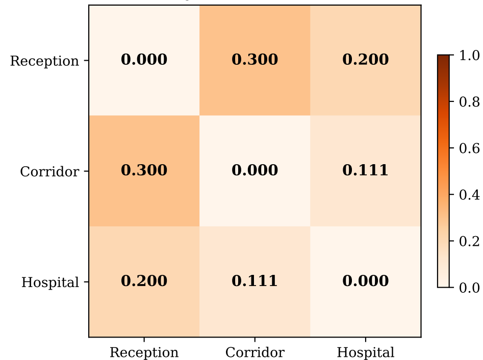
Primitive Set Divergence (Jaccard distance)
