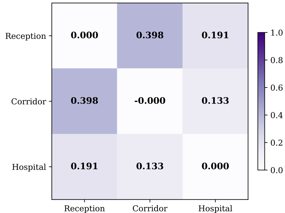
Weight Profile Distance (Cosine distance of Q(f|c) )
