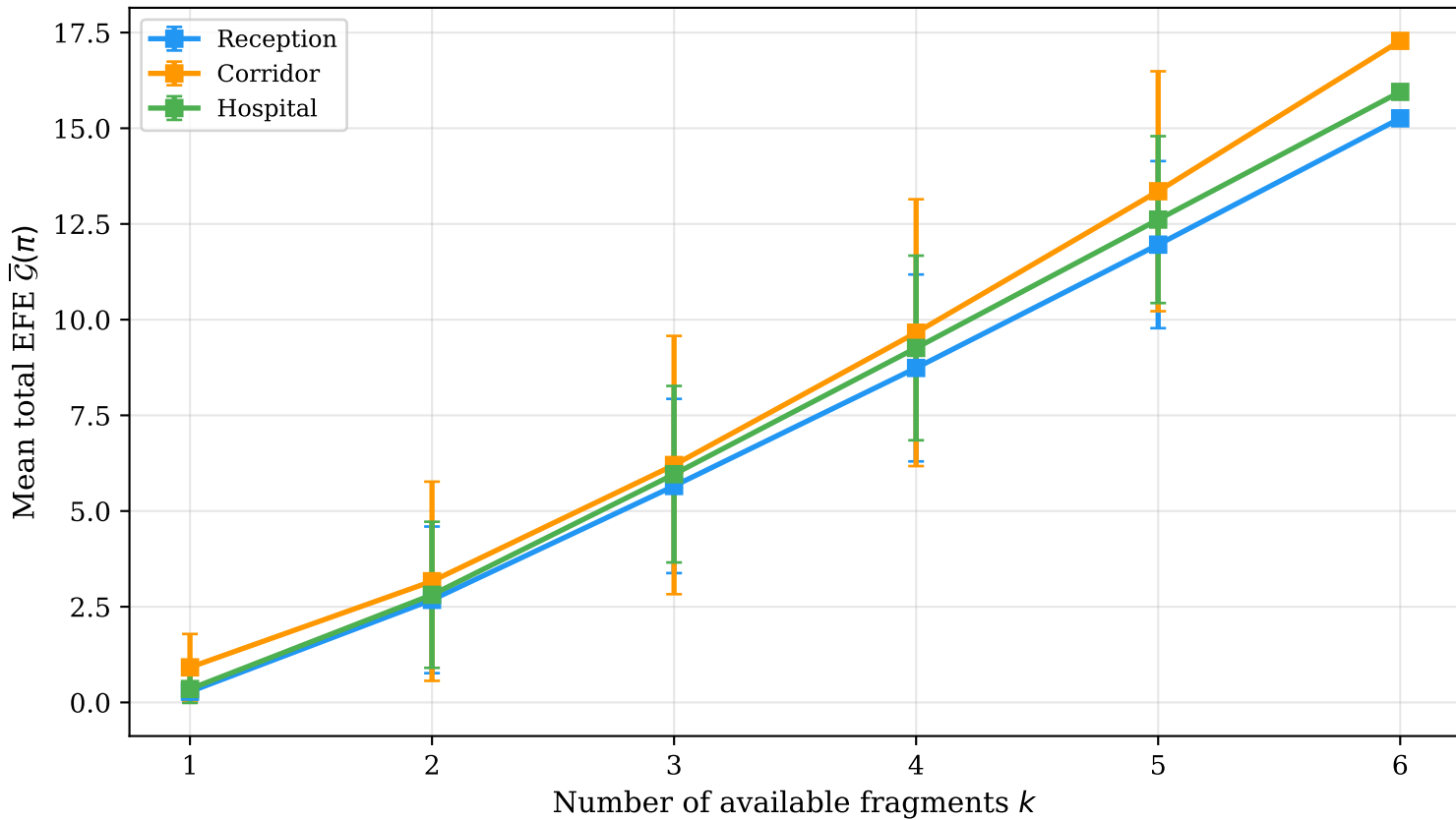
Expected Free Energy vs. Model Richness (Context preference structure creates persistent EFE separation)
