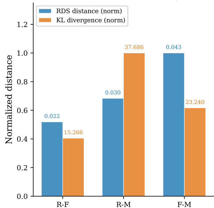
(c) RDS Distance vs KL Divergence
