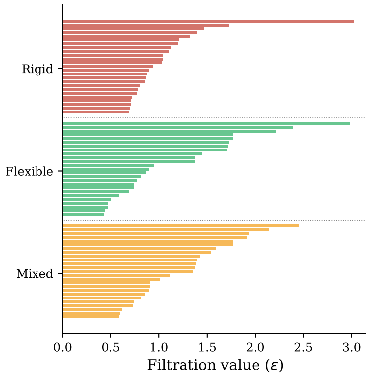
(b) H_0 Persistence Barcodes
