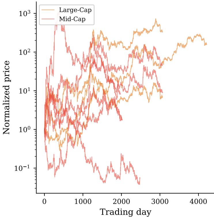
(a) Crypto Price Trajectories
