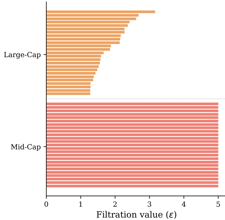
(b) H_0 Persistence Barcodes
