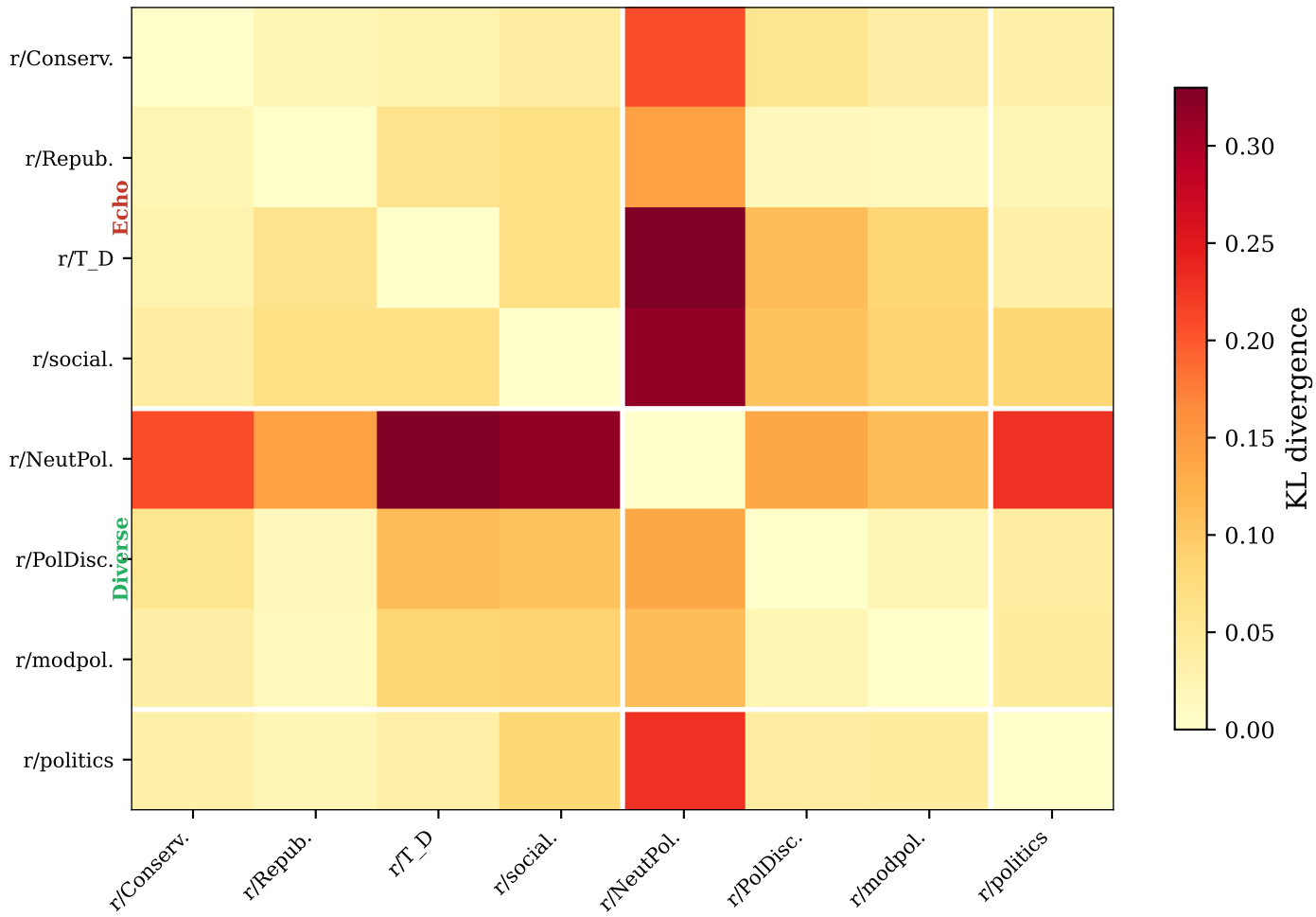
(a) KL Divergence (discrimination ratio = 1.70)
