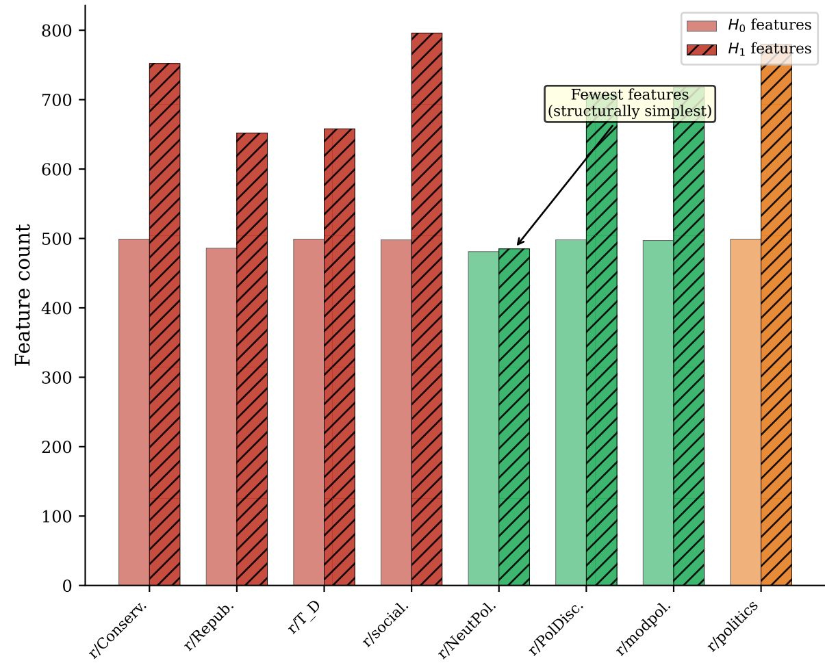
(b) Persistent Homology Features
