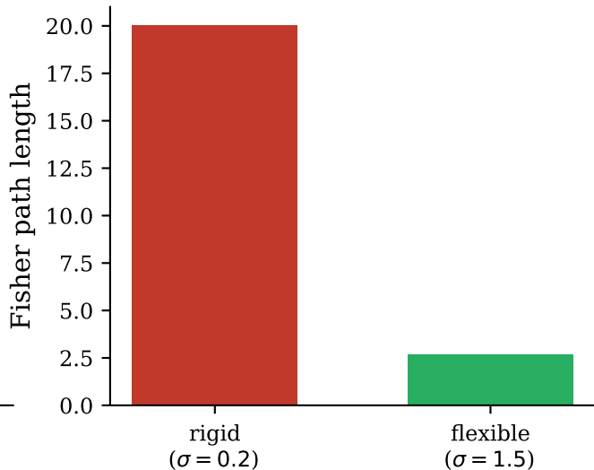
Cost of the same belief change
