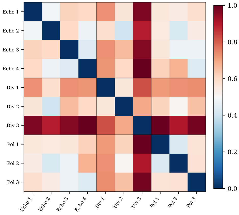
RDS Distance
