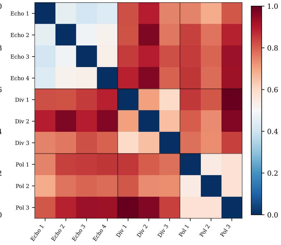
Embedding Distance
