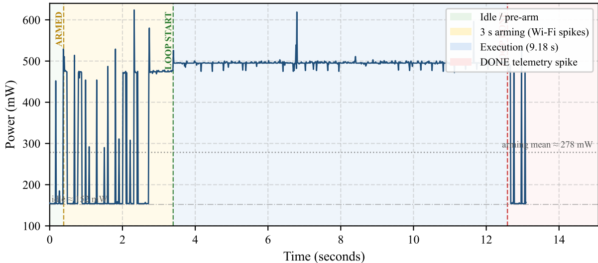
ESP8266 warm-cache energy run (1,000,000 lookups) — loop 9.18 s
