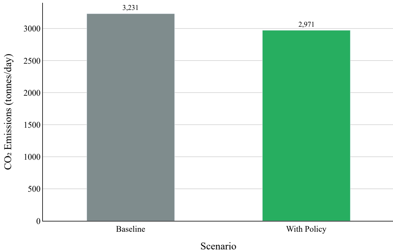
Figure 2. Daily CO 2 Emissions (Reduction: 8.0%)
