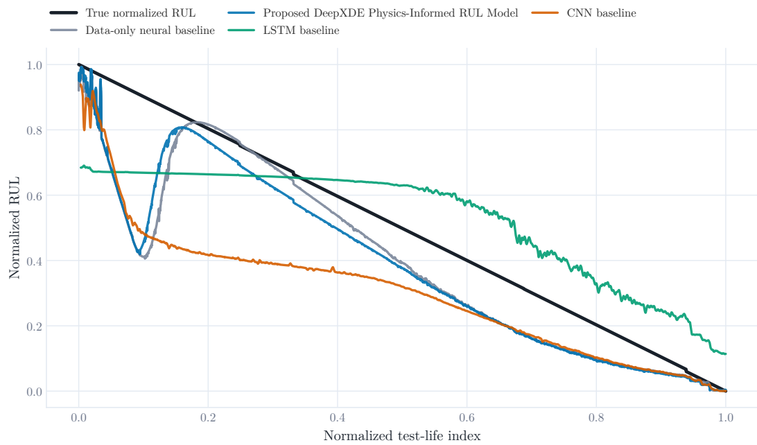
Figure 5.14: Experiment 2 true and predicted normalized RUL on the held-out test run.
