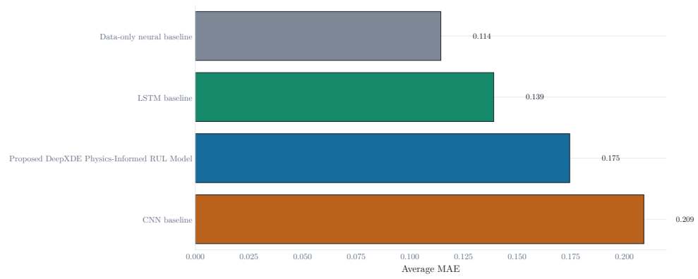
Figure 5.6: Average MAE by model across the three experiments.
