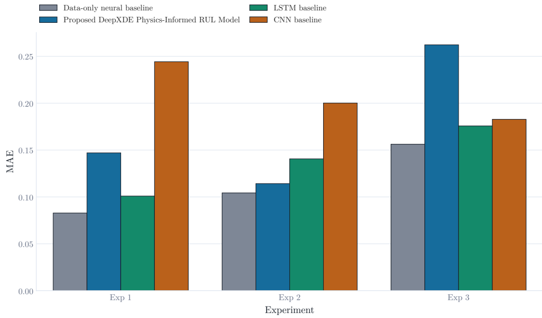
Figure 5.11: MAE by model and experiment.
