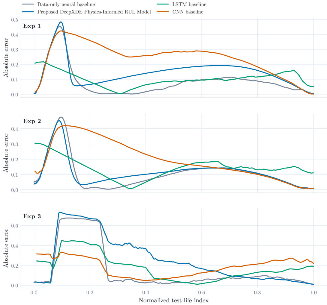
Figure 5.16: Smoothed absolute prediction error over normalized test life.
