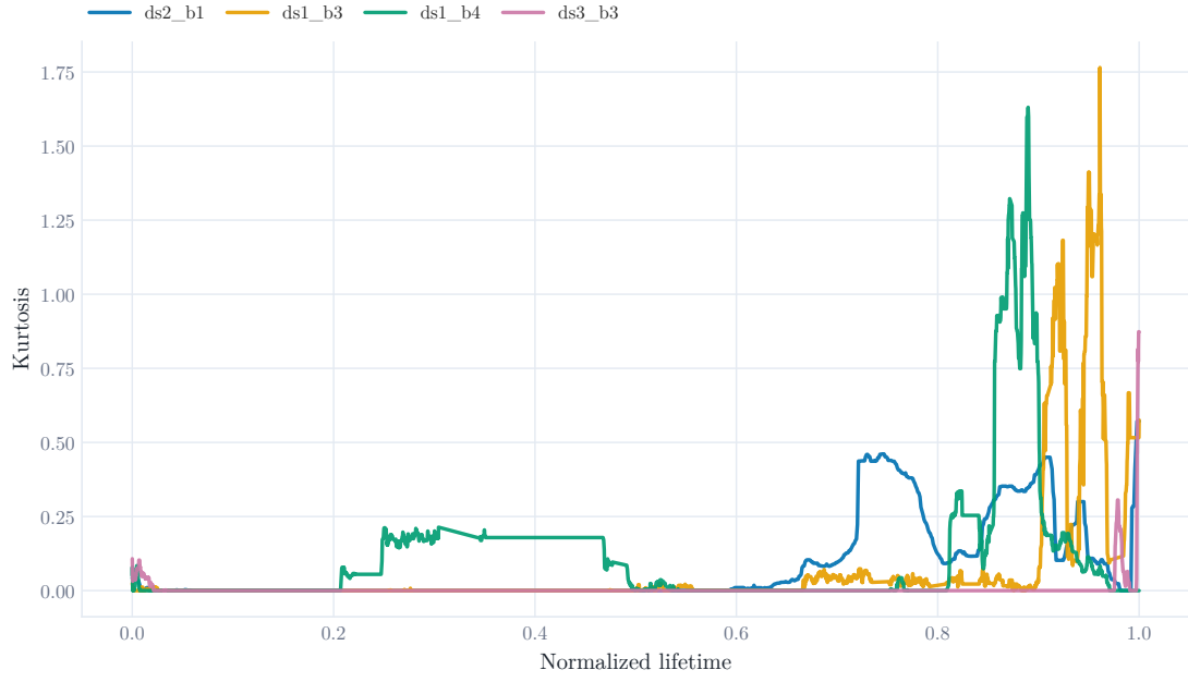
Figure 5.2: Kurtosis evolution over normalized bearing life.
