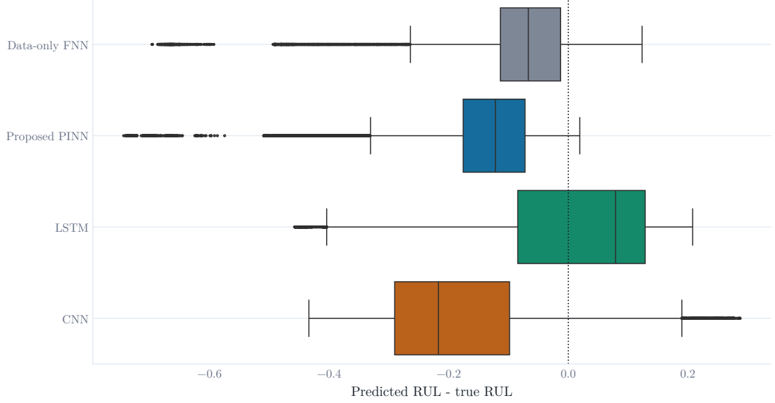
Figure 5.17: Signed prediction error distribution. Positive error means the model overestimated normalized RUL.
