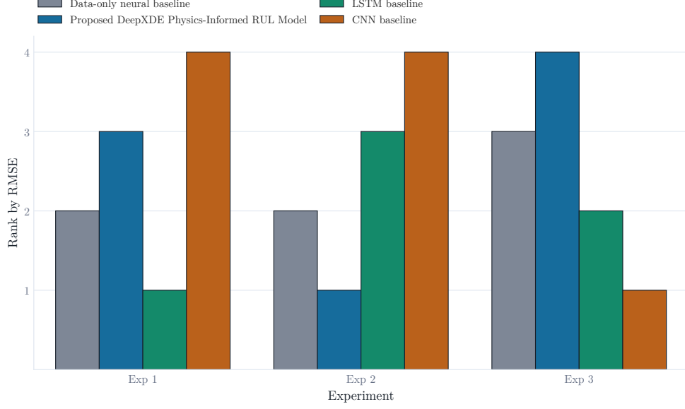
Figure 5.8: Model ranking by RMSE for each experiment. Lower rank is better.
