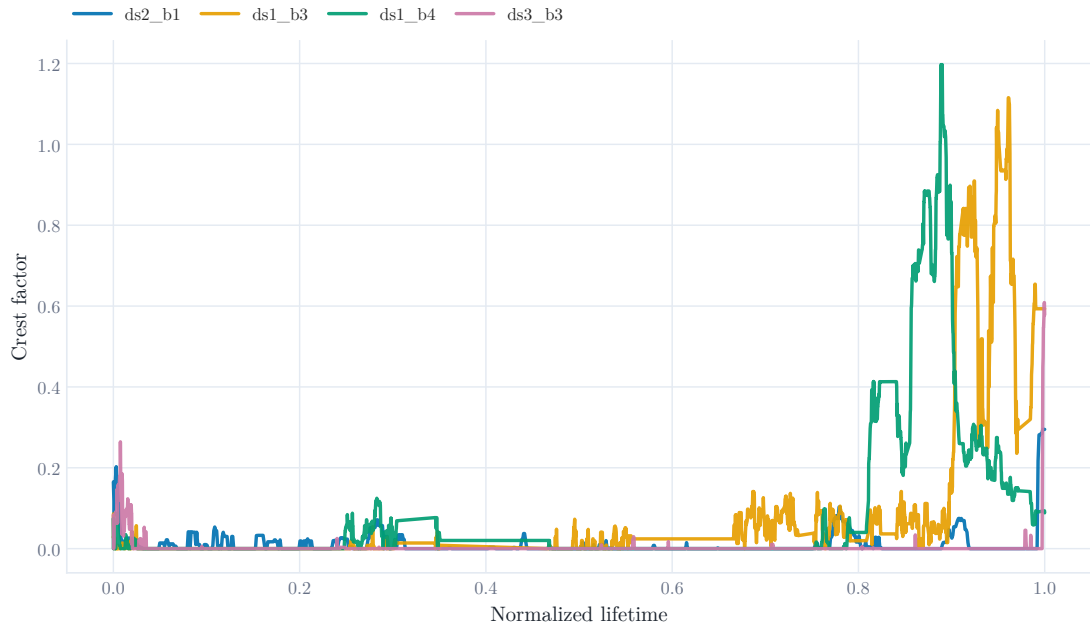
Figure 5.3: Crest factor evolution over normalized bearing life.
