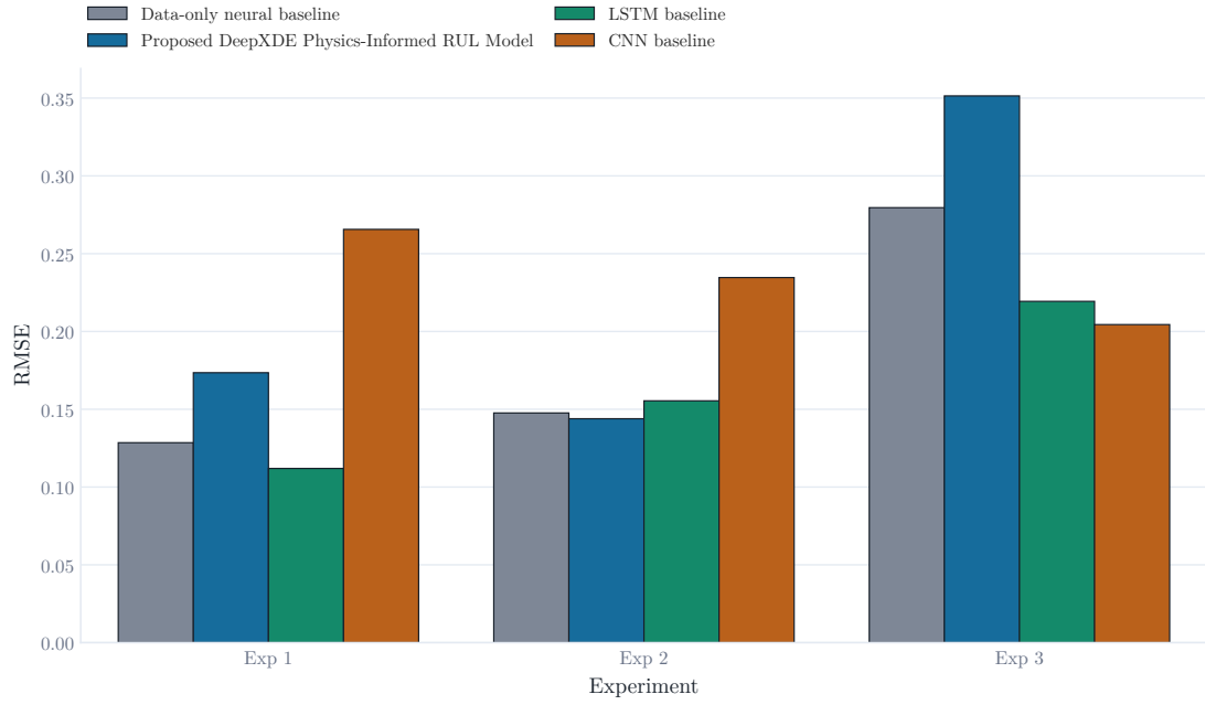
Figure 5.10: RMSE by model and experiment.
