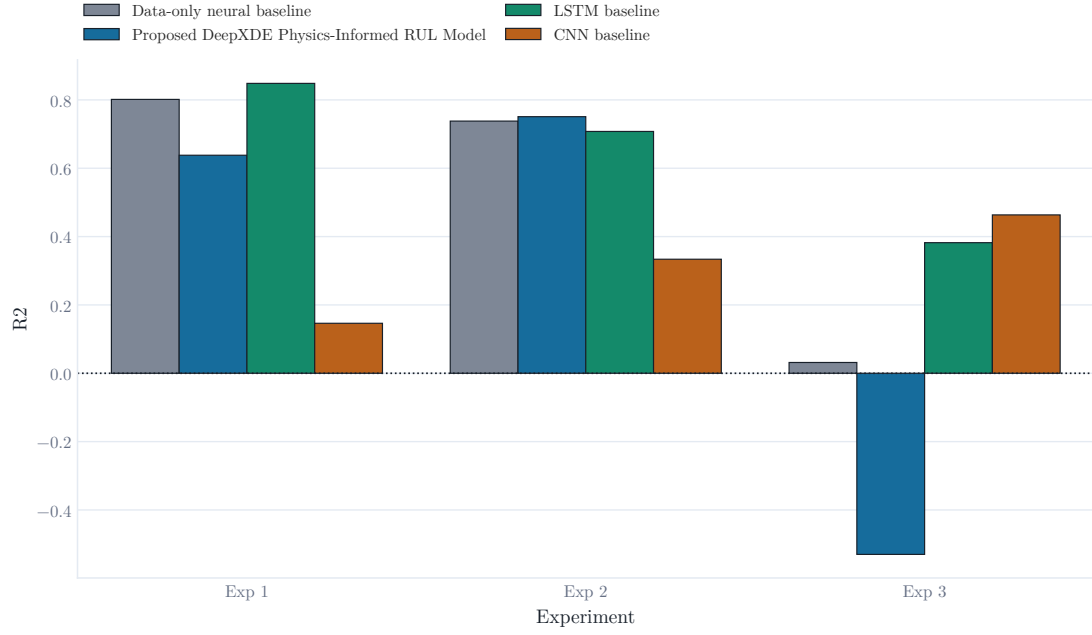
Figure 5.12: R^2 by model and experiment.
