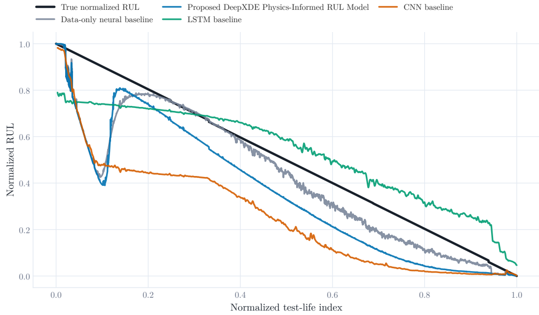
Figure 5.13: Experiment 1 true and predicted normalized RUL on the held-out test run.
