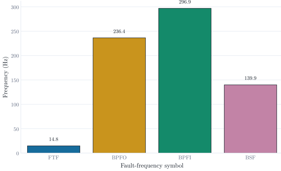
Figure 3.4: Bearing fault-frequency values used as markers for envelope spectral-energy extraction.
