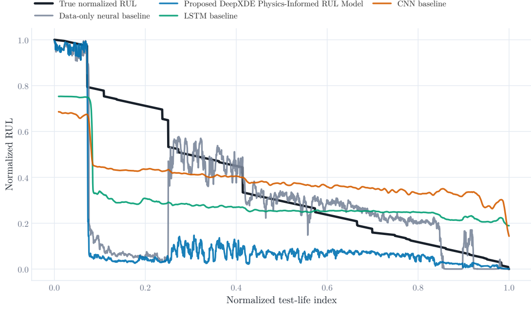
Figure 5.15: Experiment 3 true and predicted normalized RUL on the held-out test run.
