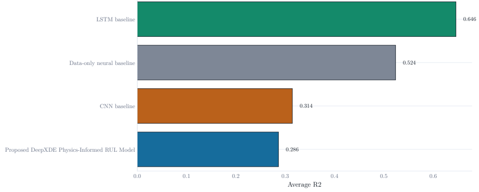
Figure 5.7: Average R^2 by model across the three experiments.
