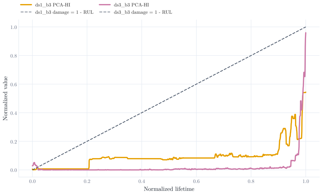
Figure 3.5: Smoothed PCA health indicator compared with normalized damage on held-out test runs.
