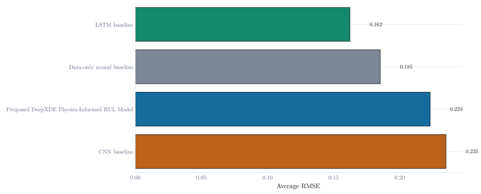
Figure 5.5: Average RMSE by model across the three experiments.
