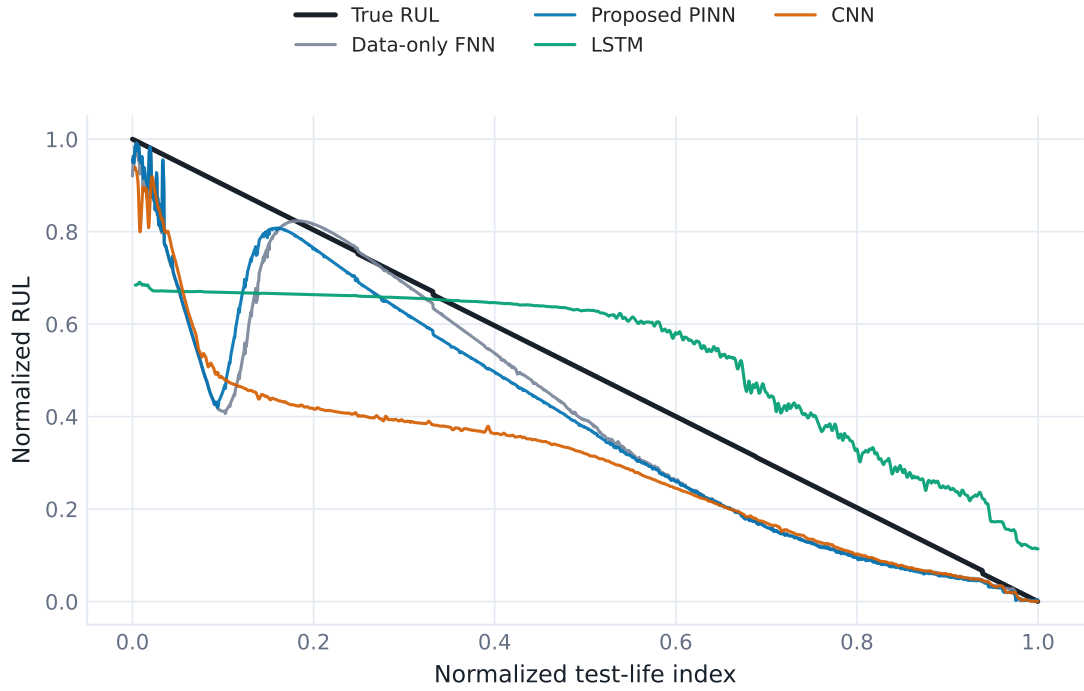
Figure 5.15: Experiment 2 true and predicted normalized RUL on the held-out test run.
