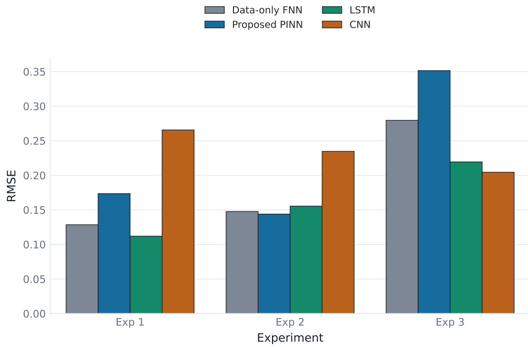
Figure 5.11: RMSE by model and experiment.
