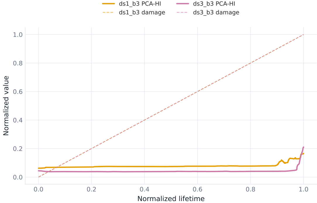
Figure 3.4: Smoothed PCA health indicator compared with normalized damage on held-out test runs.
