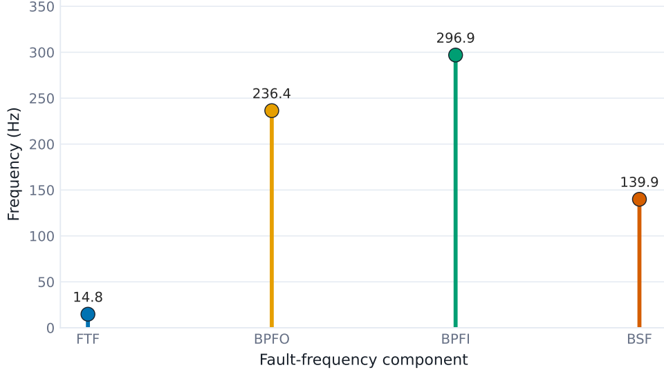
Figure 3.3: Bearing fault-frequency values used as markers for envelope spectral-energy extraction.
