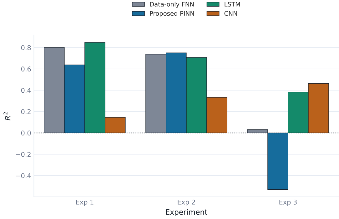
Figure 5.13: R^2 by model and experiment.
