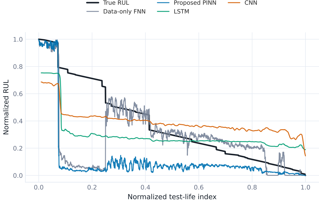
Figure 5.16: Experiment 3 true and predicted normalized RUL on the held-out test run.
