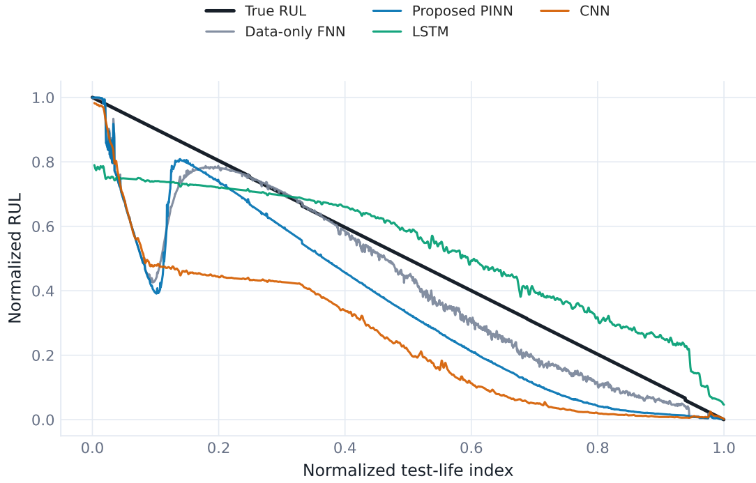
Figure 5.14: Experiment 1 true and predicted normalized RUL on the held-out test run.
