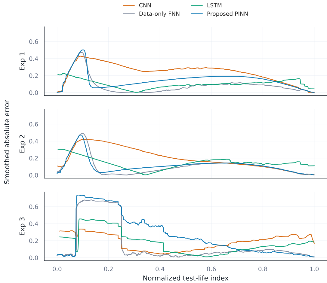
Figure 5.17: Smoothed absolute prediction error over normalized test life.
