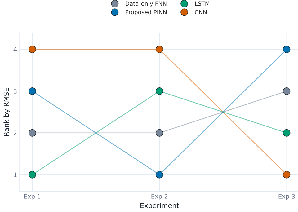
Figure 5.9: Model ranking by RMSE for each experiment. Lower rank is better.
