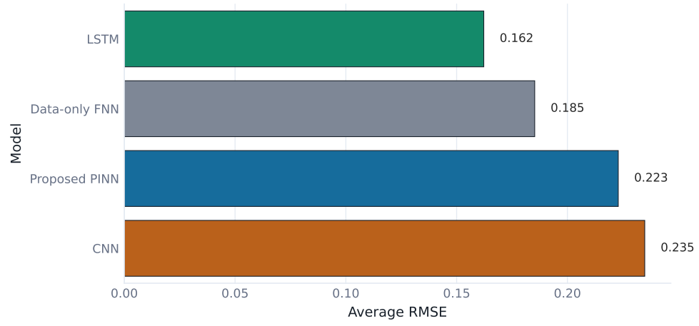
Figure 5.6: Average RMSE by model across the three experiments.
