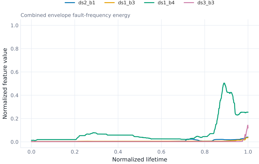
Figure 5.4: Combined fault-frequency envelope energy evolution over normalized bearing life.
