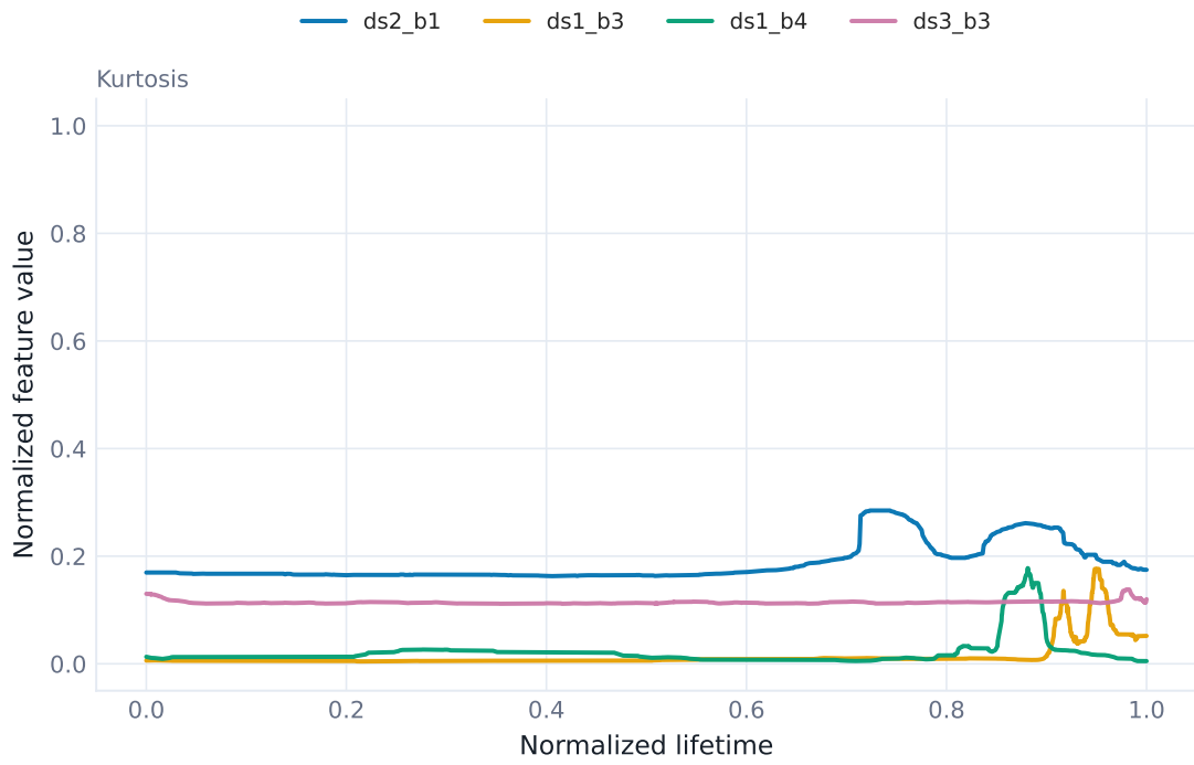
Figure 5.2: Kurtosis evolution over normalized bearing life.
