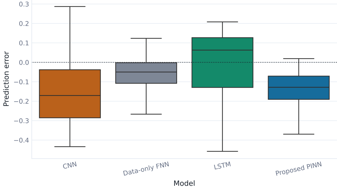
Figure 5.18: Signed prediction error distribution. Positive error means the model overestimated normalized RUL.
