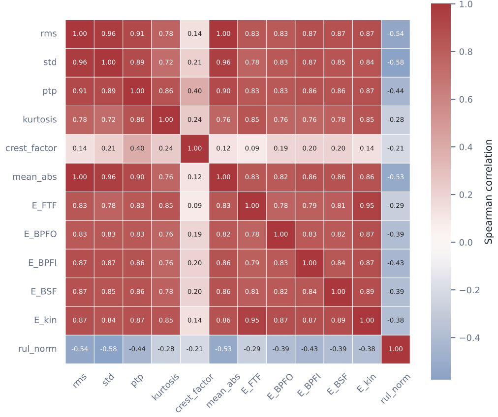
Figure 5.5: Spearman correlation structure of extracted features and normalized RUL.
