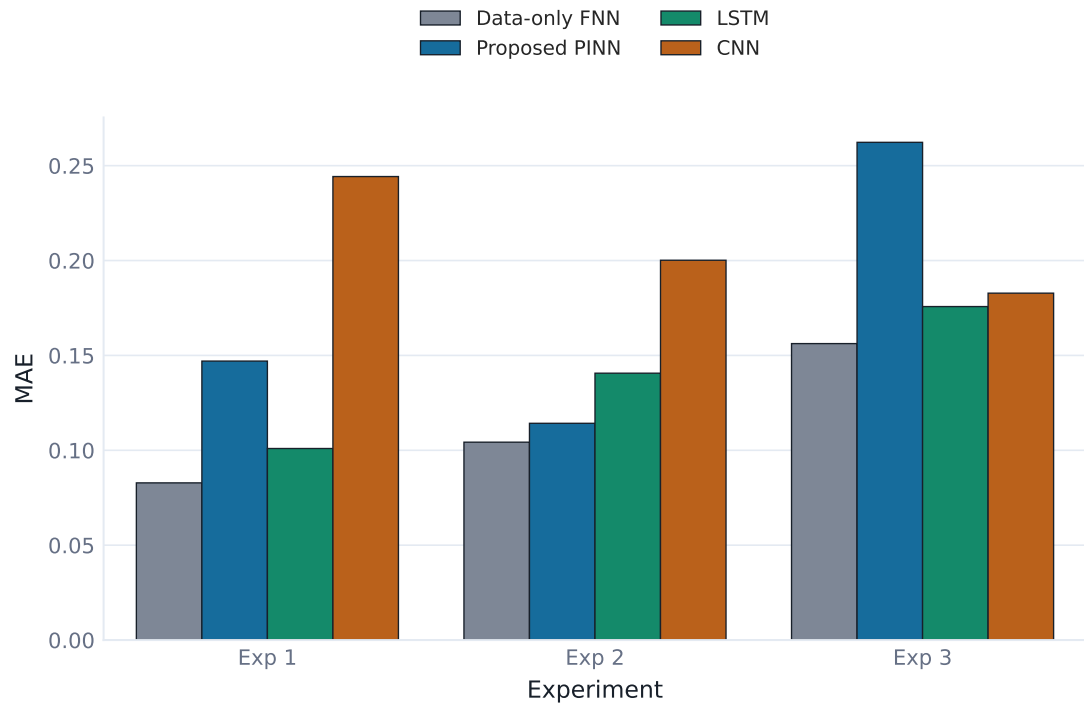
Figure 5.12: MAE by model and experiment.
