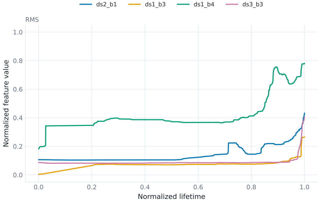
Figure 5.1: RMS evolution over normalized bearing life.
