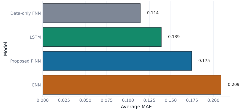
Figure 5.7: Average MAE by model across the three experiments.
