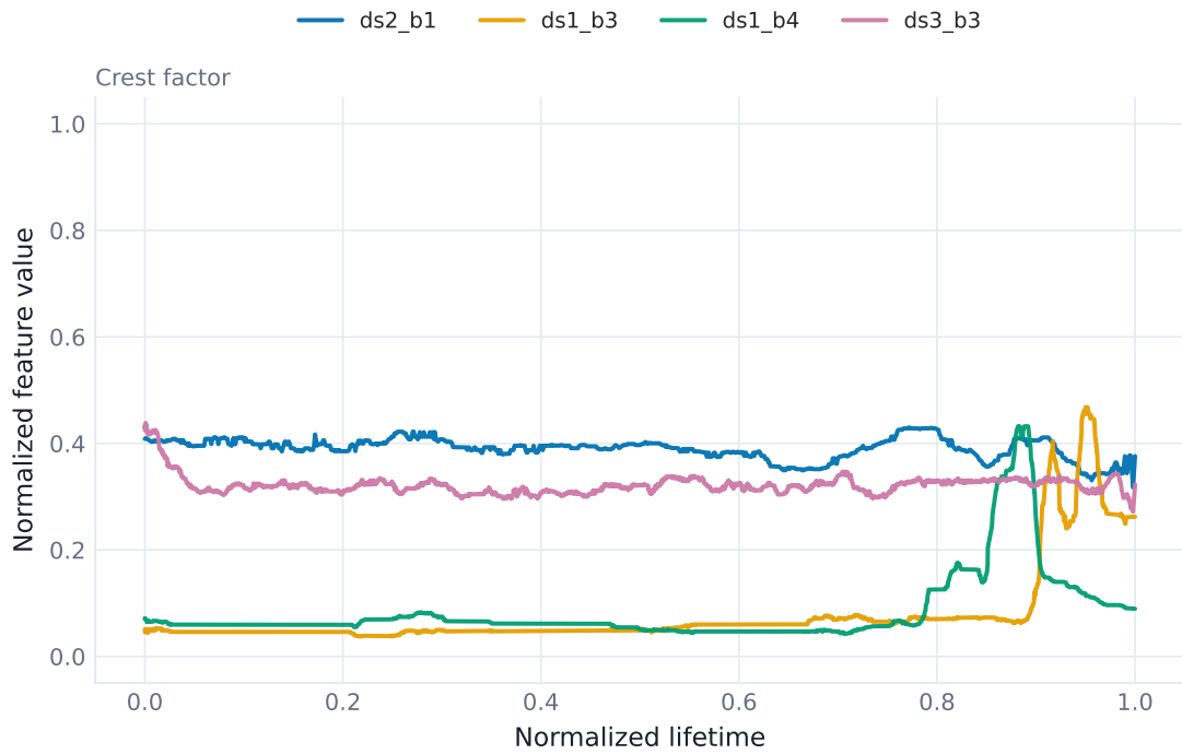
Figure 5.3: Crest factor evolution over normalized bearing life.
