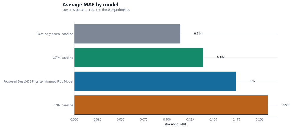
Figure 5.6: Average MAE by model across the three experiments.
