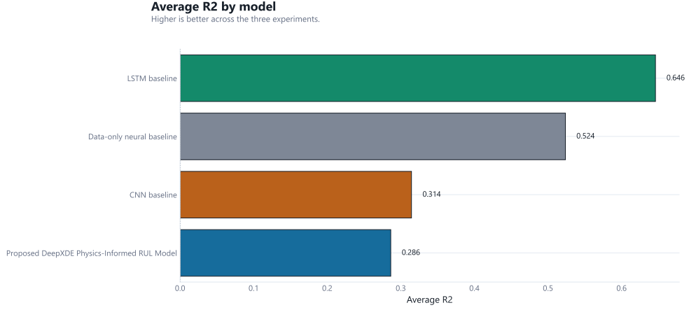
Figure 5.7: Average R^2 by model across the three experiments.
