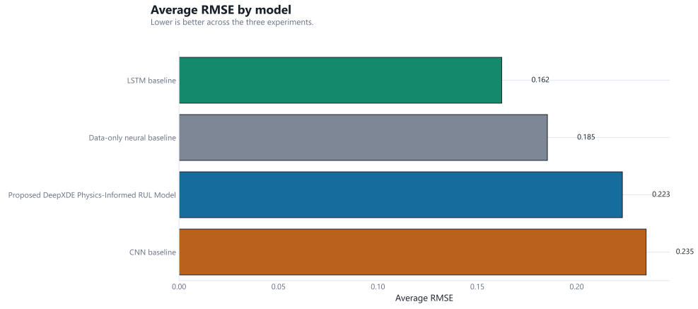
Figure 5.5: Average RMSE by model across the three experiments.
