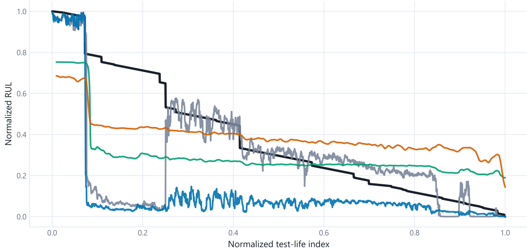
Figure 5.15: Experiment 3 true and predicted normalized RUL on the held-out test run.
