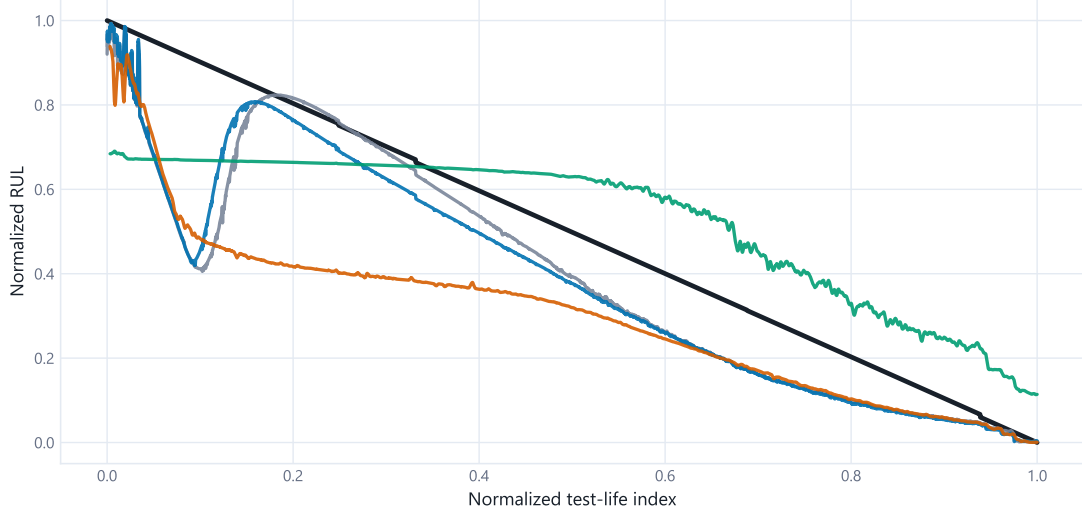
Figure 5.14: Experiment 2 true and predicted normalized RUL on the held-out test run.
