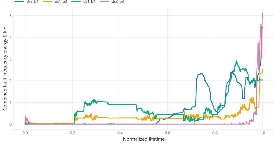
Figure 5.4: Combined fault-frequency envelope energy evolution over normalized bearing life.
