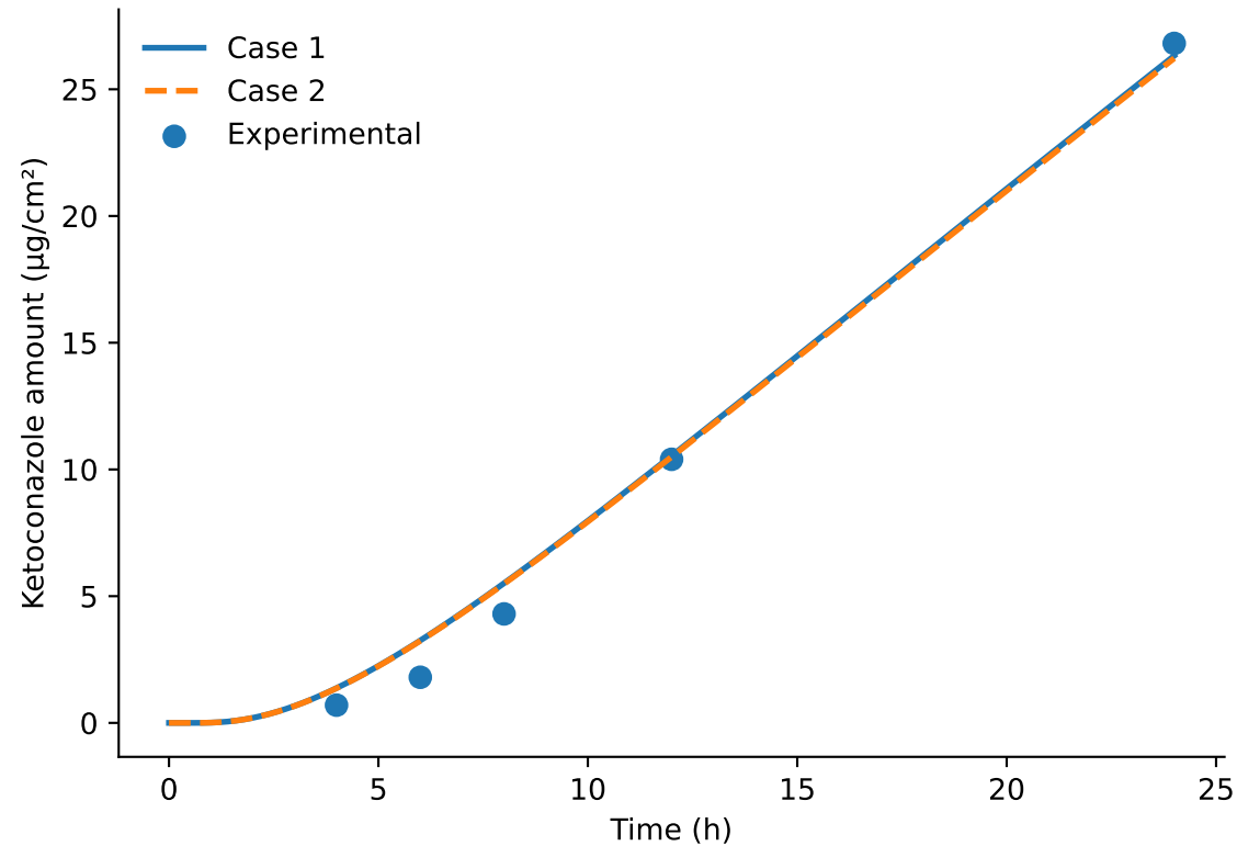
Free KC receptor fit comparison
