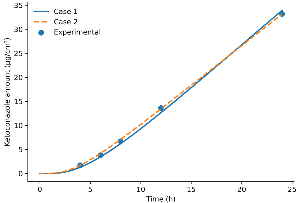
KLZ-NPs receptor fit comparison
