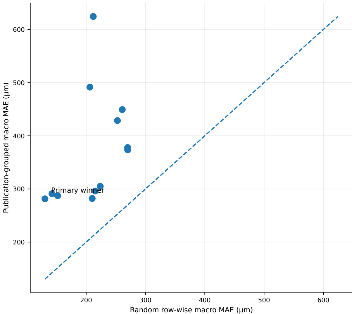
Filament diameter: validation optimism
