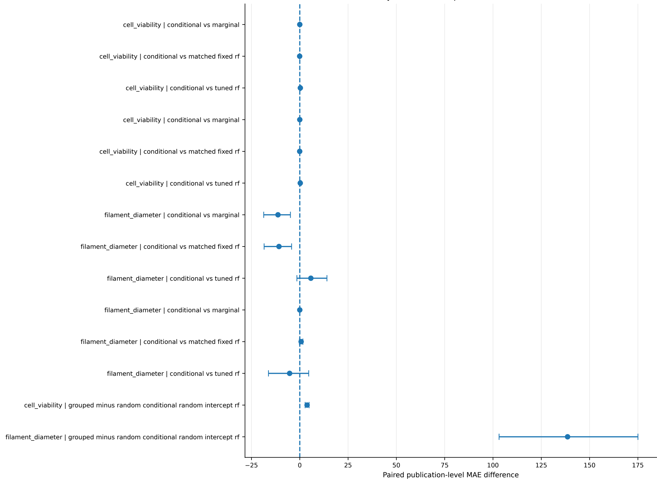
Confirmatory random-intercept Random Forest contrasts
