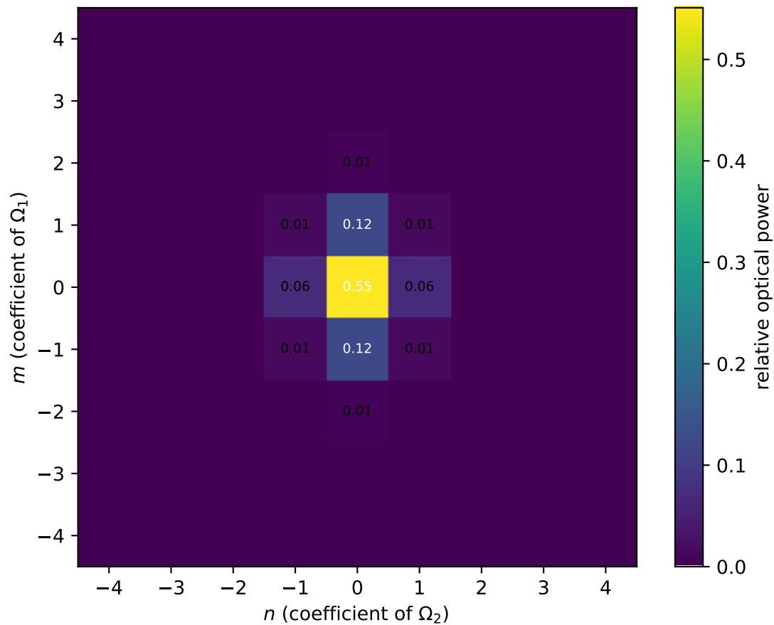
Two-tone phase modulation: optical sideband lattice \omega_0 + m\Omega_1 + n\Omega_2
